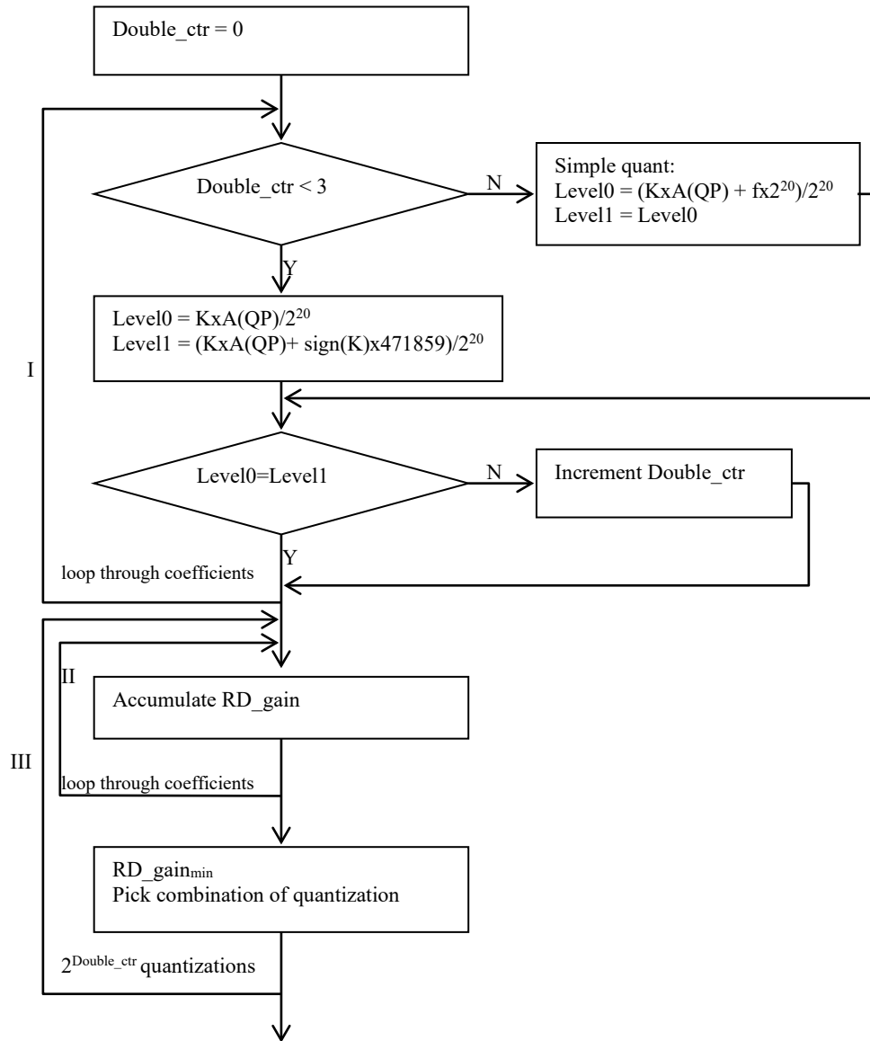
Figure 8 Block diagram of RD-quant
