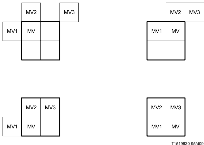
FIGURE F.1/H.263 Redefinition of the candidate predictors MV1, MV2 and MV3 for each of the luminance blocks in a macroblock
