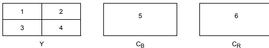
FIGURE 5/H.263 Arrangement of blocks in a macroblock
