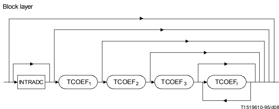
FIGURE E.1/H.263 Structure of SAC Block layer
