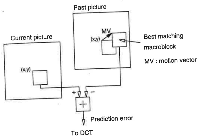
Figure 6.6 Forward motion compensation.
