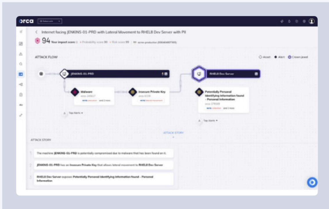
ORCA DISPLAYS ATTACK PATHS VISUALLY
