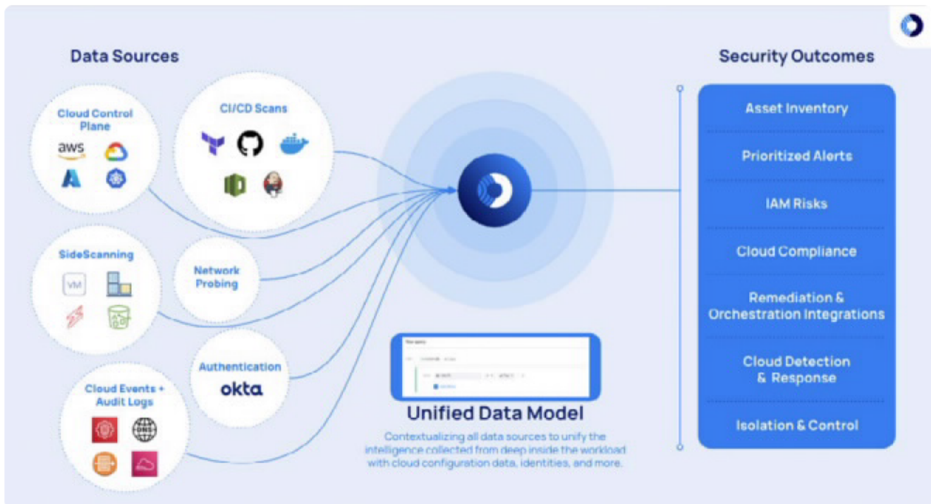
DIAGRAM OF ORCA'S UNIFIED DATA MODEL
