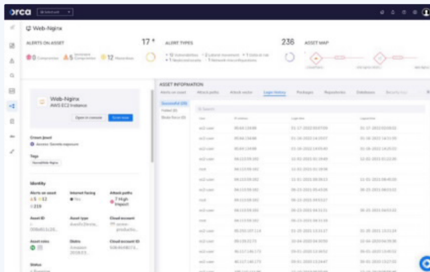
ORCA SHOWS ALL ASSET INFORMATION, INCLUDING FILE INTEGRITY
