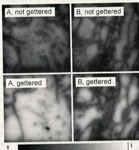
FIG. 2. Spatially resolved PL image of two passivated, emitter-free mc-Si neighboring wafers before and after annealing at 850 °C for 30 min.
