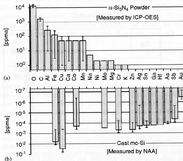
Fig. 1. (a) Vendor-specified impurity contents of four different commercially available \alpha - \text{Si}_3\text{N}_4 powders with purities between 95% and 99.9%. The range of variation, which depends on the purity of the powder, is shown by the error bars. (b) Impurity content of different directionally solidified ingot-grown mc-Si materials determined by NAA [1–3]. The error bars show the range of values obtained on different samples.
