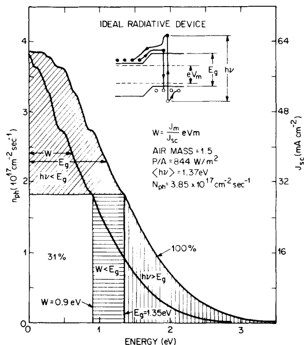
FIG. 2. Graphical analysis of the efficiency of an ideal solar cell. The outer curve is E_g versus n_{ph} , the absorbed photon flux. The inner curve is W , the work per absorbed photon versus n_{ph} . The area under the outer curve is the solar power per unit area. The shaded areas equal different losses as explained in the text. The unshaded area is the power per unit area delivered to the load.
