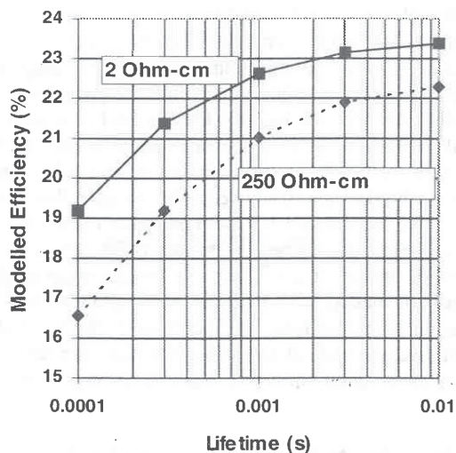
Fig. 4: Influence of carrier lifetime on the efficiency of Backside-Contact cells for low- and high-resistivity silicon substrates.
