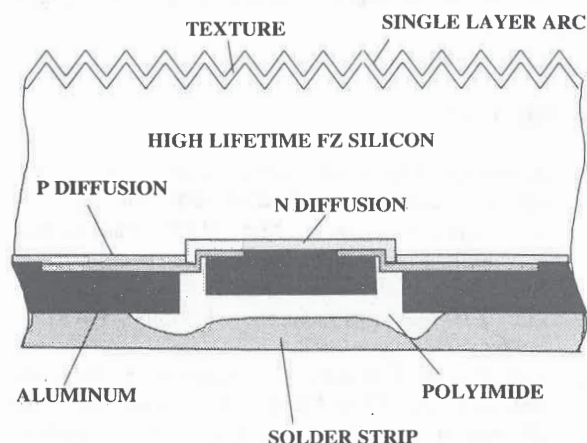
Fig. 1: Cross section of a Backside-Contact solar cell.
