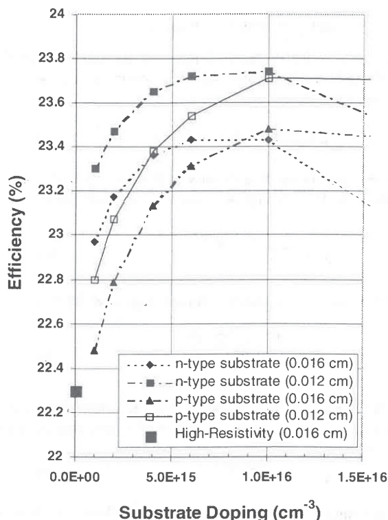
Fig. 3: Efficiency of Backside-Contact cells vs. Substrate doping level for N and P-type substrates, and for 120 \mu\text{m} and 160 \mu\text{m} thick cells.
