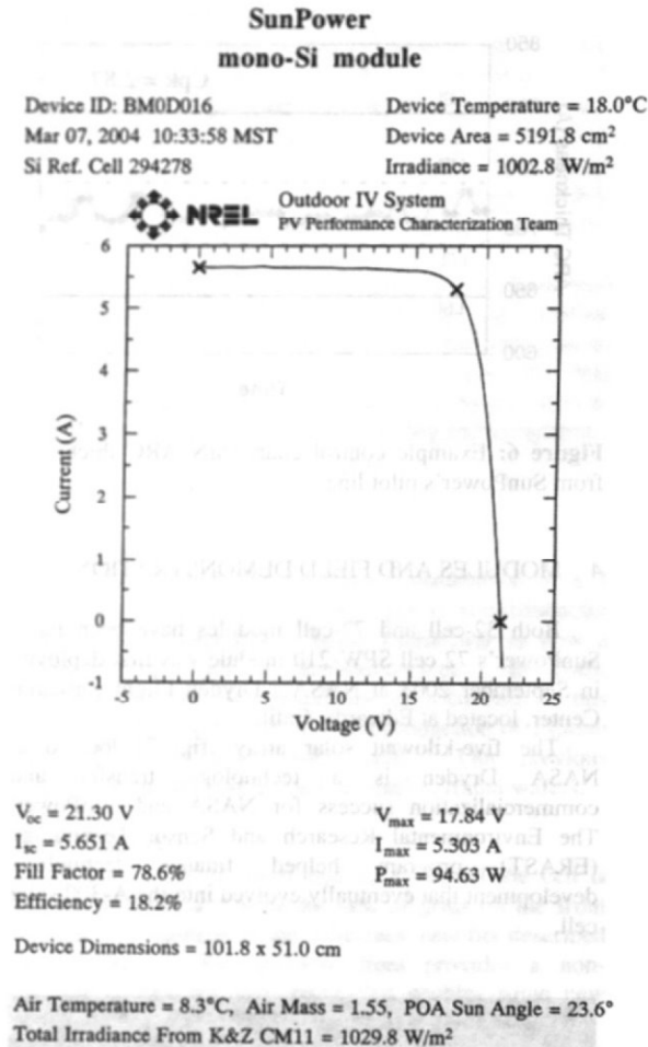
Figure 8: IV Curve 18.2% efficient 32-cell module tested by NREL.
