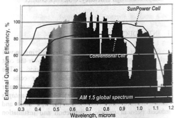
Figure 3: Spectral response of SunPower cell.
