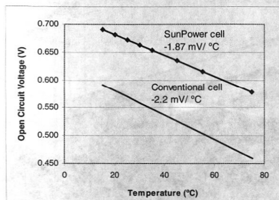
Figure 5: Temperature dependence of Voc
