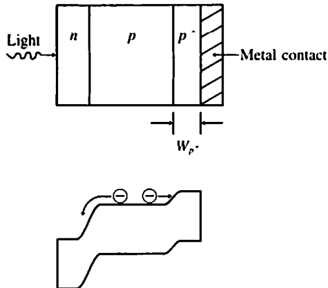
Figure 3.20 Back surface field cell. The field at the p/p^+ junction retards the flow of the electrons toward the back surface.
