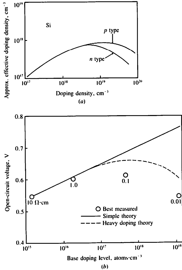
Figure 3.19 (a) The high doping effect: The effective doping density saturates or even drops with increasing doping density. (b) V_{oc} as a function of the bulk doping density. (Godlewski et al. , 1977.)
