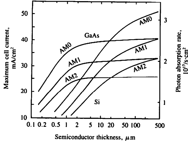
Figure 3.7 Maximum available cell current density and rate of photon absorption as function of cell thickness.
