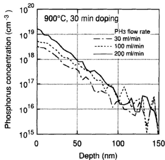
Fig. 1. SIMS profiles of phosphorus. Doping was carried out at 900°C for 30 min. \text{PH}_3 flow rate was varied from 30 to 200 ml/min.
