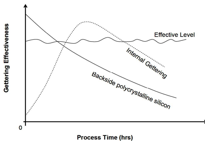
Fig. 1. Effectiveness of gettering techniques as a function of process time. During high temperature process the backside polycrystalline layer partially recrystallizes and thus loses a great part of its gettering capability. Excerpted from [4].
