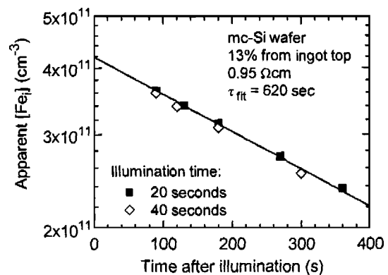
FIG. 1. Reduction in the “apparent” Fe i concentration due to repairing after illumination. The straight line shows the exponential fit used to estimate [Fe i ] immediately after illumination. Illumination times of 20 and 40 s are shown.
