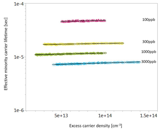
Fig. 2. Effective minority carrier lifetime vs excess carrier density at low level injection (LLI) for the liquid contamination concentrations in the range 100–3000 ppb. From the slope of the fitted curves the capture cross section is extracted.
