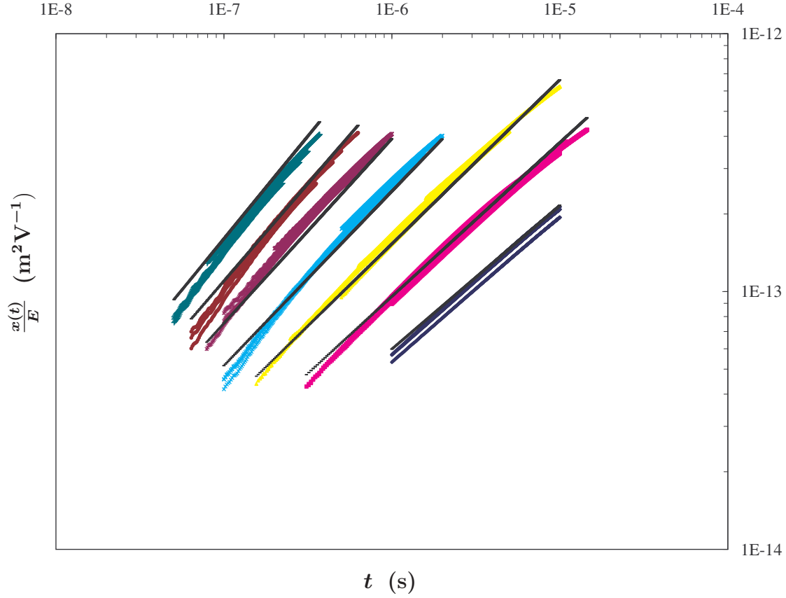
FIGURE 5.13: Displaceability curves at seven temperatures, determined from the pre-transit normalized charge traces, are simultaneously fit with Eqn (5.6). The fit, indicated at each temperature with a black line, is very good.
