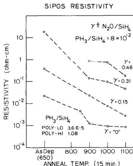
Fig. 3. N + SIPOS film resistivity vs T_A and \gamma .
