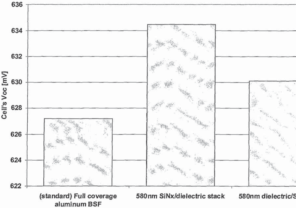
Cell's Open Circuit Voltage with different surface passivation tech
