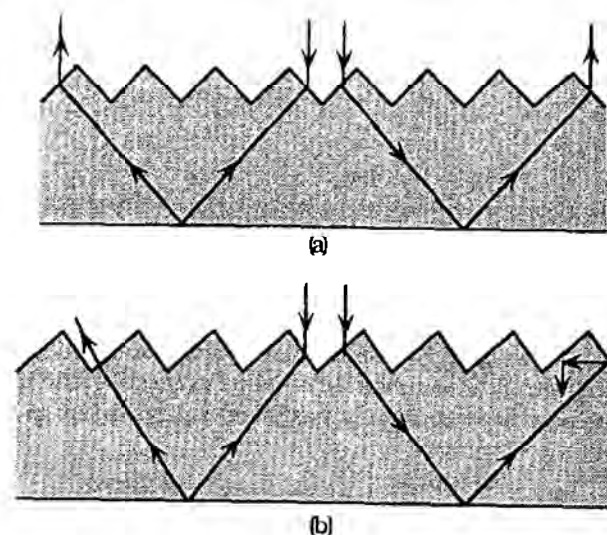
Figure 6.5: Light-trapping with top surface grooves formed by intersecting (111) equivalent planes: (a) untilted structure; (b) effect of a slight tilt.
