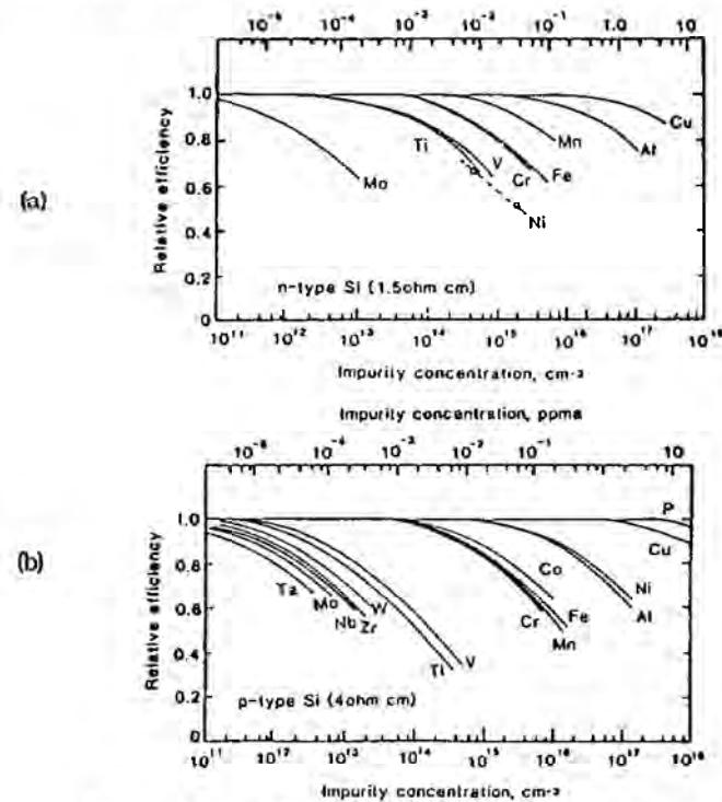
Figure 9.13: Effect of the deliberate inclusion of different concentrations of impurities upon the performance of solar cells fabricated on (a) n-type substrates (after Davis et al. [9.57]); and (b) p-type substrates (after Davis et al. [9.57]).
