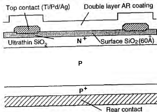
Figure 10.6: Metal-Insulator-NP junction (MINP) solar cell.
