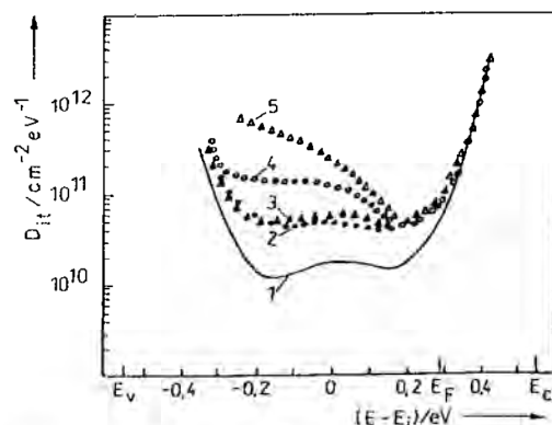
Figure 9.3: Degradation of the interface state density of Al/SiO 2 /Si and SiO 2 /Si structures by annealing (treatments in forming gas (450°C, 30 min.) and dry N 2 (500°C, 5 min). The specimens (thermally oxidized n-Si(111), 10 Ωcm) were well stabilized by a PMA process before initial measurement (curve 1). Al/SiO 2 /Si - annealed in FG (curve 2); annealed in N 2 (curve 3); SiO 2 /Si - annealed in FG (curve 4); annealed in N 2 (curve 5).
