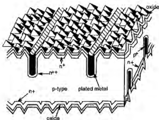
Figure 11.6: Double-sided or bifacial buried contact solar cell.
