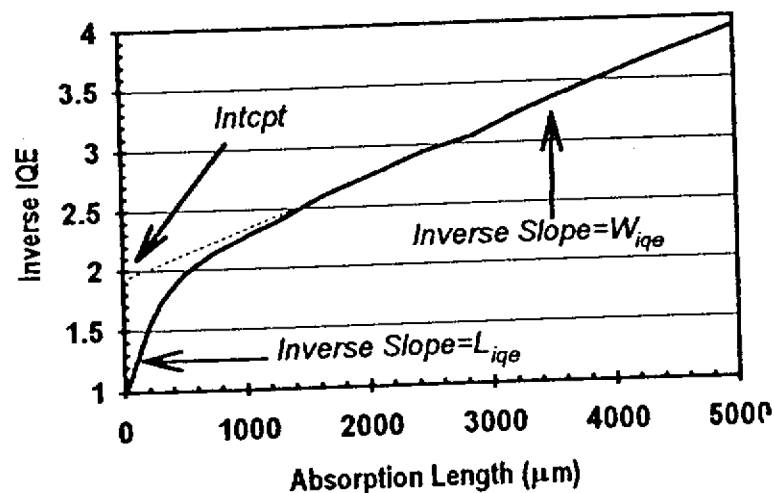
Fig. 6.14: Typical inverse internal quantum efficiency (IQE) data for an experimental cell [after Basore [6.20]].
