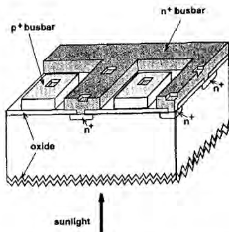
Figure 10.9: Rear point contact solar cell which demonstrated 22% efficiency in 1988 (cell rear shown uppermost).
