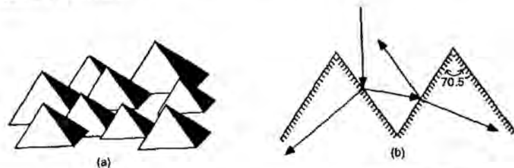
Figure 10.4: (a) Schematic diagram showing the square-based pyramids formed by exposed (111) crystallographic planes when (100)-oriented silicon wafers are anisotropically etched; (b) ray diagram showing paths of reflected and transmitted light.
