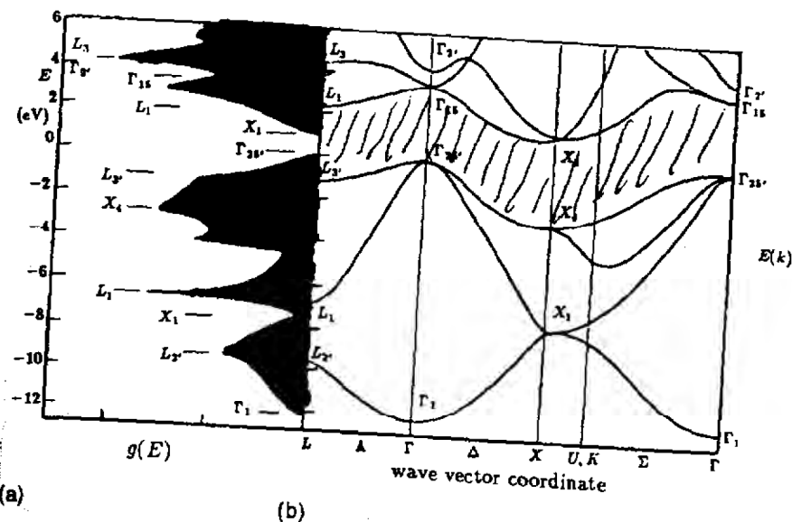
Figure 2.5: The energy band structure for silicon is shown in (b) as calculated using an empirical non-local pseudopotential scheme with the associated density of electron states g(E) shown in (a) (after Chelikowsky and Cohen [2.11] and Böer [2.12]).
