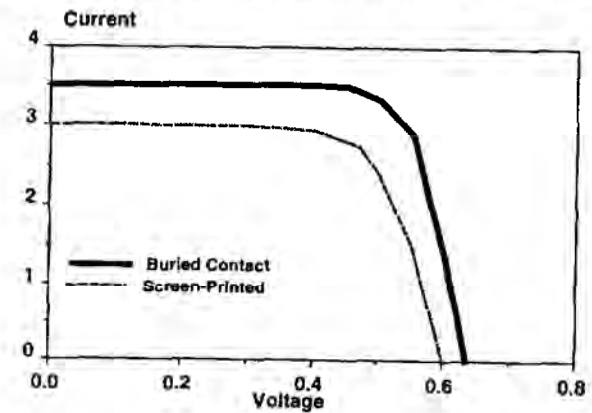
Figure 11.5: Output characteristics of buried contact cells compared to screen printed cells [after 11.15].
