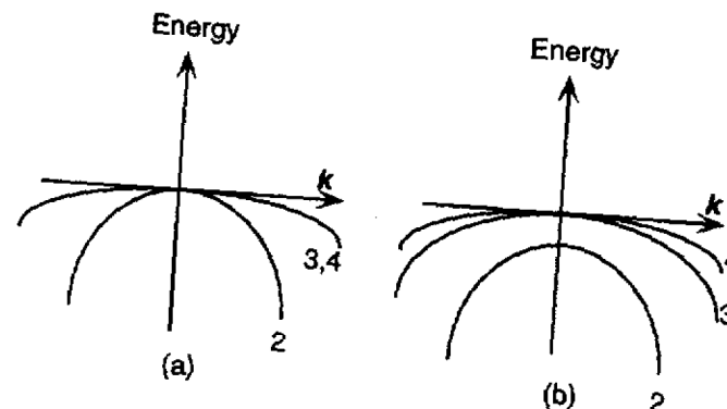
Figure 2.8: Effect of spin-orbit splitting on the three uppermost valence bands near k = 0 : (a) without spin-orbit splitting; (b) with spin-orbit splitting.
