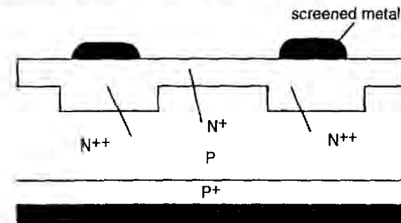
Figure 11.3: Ideal situation for fine linewidth screen printed metallization with contact being made to selectively doped areas.
