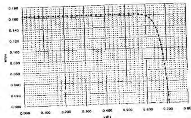
Figure 10.11: Output characteristics of a 24% efficient PERL cell.
