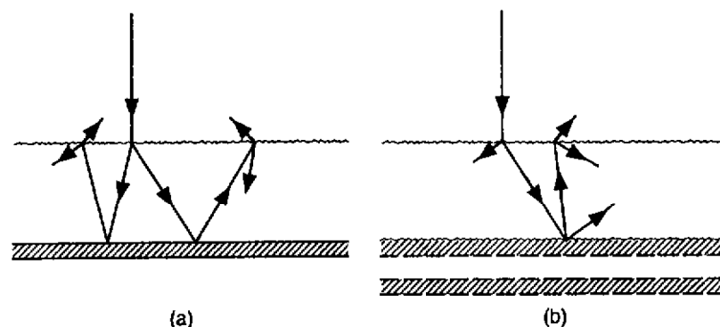
Figure 6.2: Other randomizing light trapping schemes; (a) planar rear surface; (b) both surfaces randomizing. The broken lines at the rear surface indicate two different locations of the rear reflector
