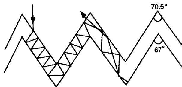
Figure 6.6: Near-parallel double-sided slat approach. Effective device thickness could best be defined as cells aperture area divided by volume [6.11].
