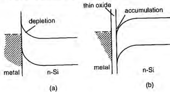
Figure 9.10: (a) Metal-silicon contact showing Schottky barrier formation; (b) metal-thin insulator-semiconductor (MIS) contact with metal work function chosen so as to cause accumulation of the semiconductor in the contact region.
