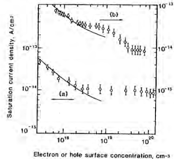
Figure 9.9: Measured values of the saturation current density associated with recombination at the p-type silicon-oxide interface as a function of the electrostatically induced (a) electron and (b) hole concentrations at this interface. The solid curves are theoretical curves, based upon a particular band-gap narrowing model (after Yablonovitch et al. [9.36]).
