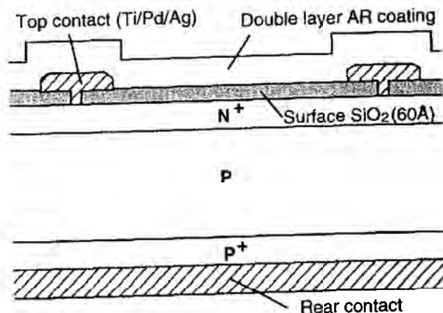
Figure 10.7: Schematic diagram of the Passivated Emitter Solar Cell (PESC cell).
