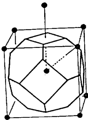
Figure 2.3: Construction of the truncated octahedron corresponding to the first Brillouin zone of the body centred cubic reciprocal lattice, showing its relationship to the cubic unit cell of this lattice.
