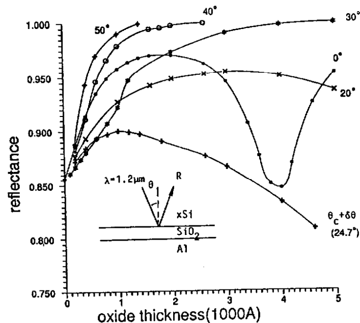
Figure 6.3: Calculated reflectance from a rear Al reflector at the rear of a silicon wafer as a function of the thickness for an intervening layer of \text{SiO}_2 , for various internal angles of incidence. The reflectance for the \theta_c + \delta\theta case reaches a minimum for about 1 mm oxide thickness (not shown), then increases towards unity (after Campbell [6.6]).
