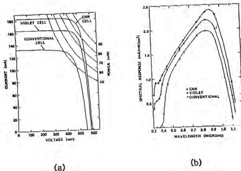
Figure 10.5: (a) Output current-voltage characteristics of a black (Comsat Non-Reflecting/CNR), a violet and a conventional solar cell under AM0 radiation; (b) spectral response of a black (CNR), a violet and a conventional cell, all of 2 cm x 2 cm dimensions [after Haynos et al [10.23]].
