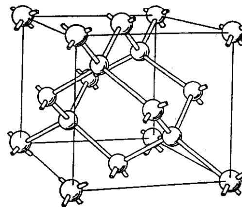
Figure 2.1: Lattice Structure of Silicon.
