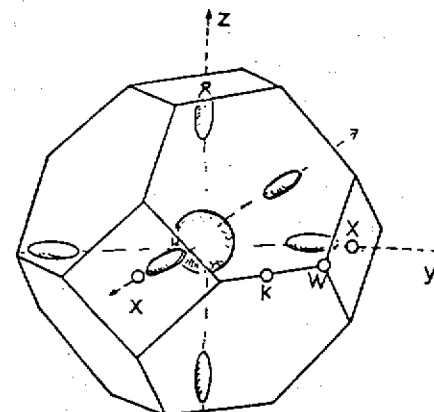
Figure 2.7: Constant energy surfaces within the Brillouin for an energy just above the conduction band minima (ellipsoids) and just below the valence band maximum (sphere).
