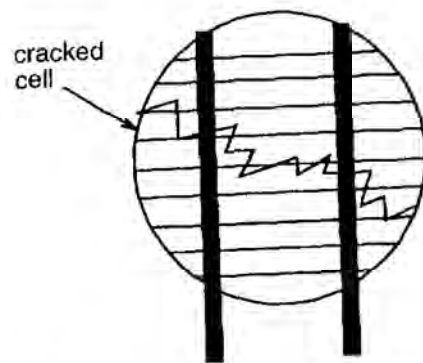
Figure 11.2: Cell design using the strip metal cell interconnects as busbars to reduce finger resistive losses and to improve tolerance to cracks.
