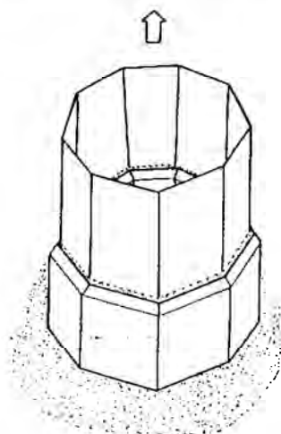
Figure 13.1: Growth of a nonagonal ribbon of silicon using the edge-defined film-fed growth (EFG) method [13.4].
