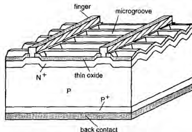
Figure 10.8: The microgrooved PESC cell, the first silicon cell to exceed 20% efficiency in 1985.
