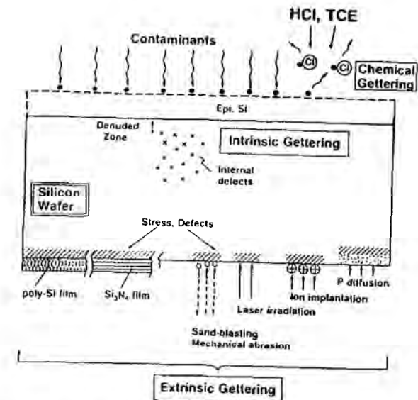
Figure 9.14: Schematic illustration showing various gettering techniques for a silicon wafer (after [9.59]).
