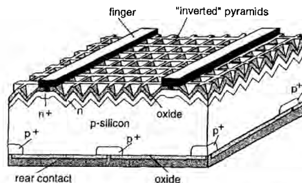
Figure 10.10: The PERL cell which took efficiency above 24% in the early 1990's.
