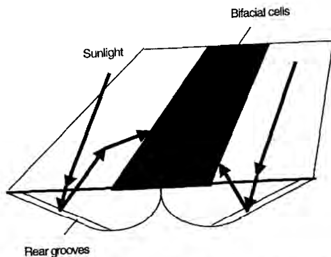
Figure 6.20: Simple static concentrator based on light trapping in "encapsulant".
