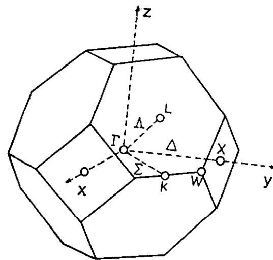
Figure 2.4: The First Brillouin Zone of the Reciprocal Lattice for Silicon.
