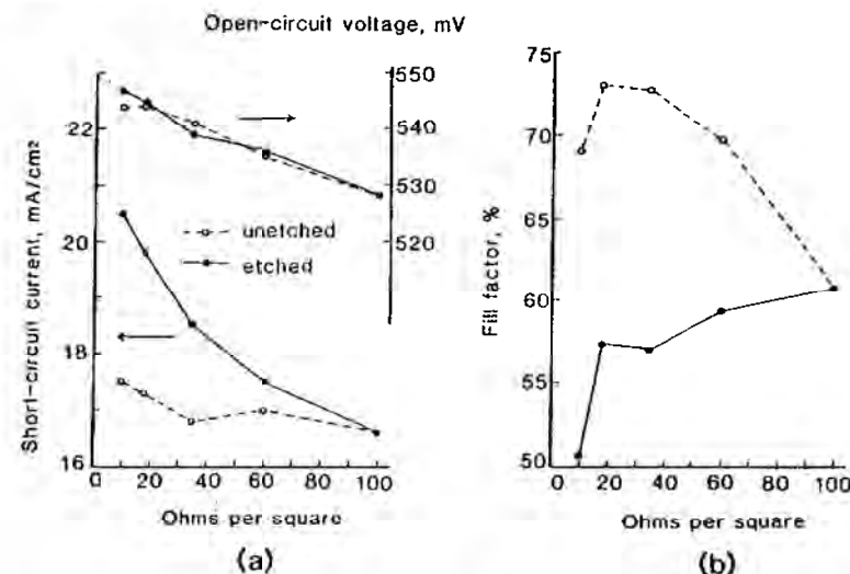
Figure 13.3: Effect of etching after diffusion upon the characteristics of multicrystalline cells. The dashed lines show the cell performance without etching, while the solid curves show the effect of etching to a sheet resistivity of 100 \Omega/\text{square} after diffusion (after Wenham [13.18]).
