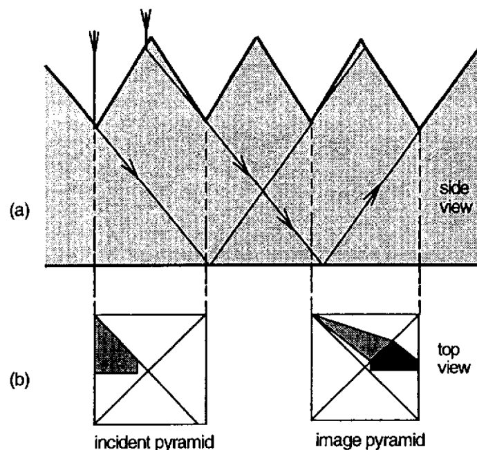
Figure 6.7: Major ray paths in regular pyramid layout: (a) side view; (b) "image region" where rays resurface.
