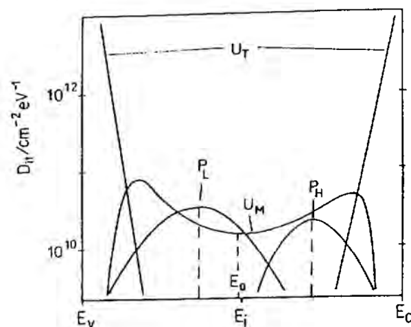
Figure 9.1: Groups of states at the Si/SiO 2 interface and their contribution to the interface state density, D_{it}(E) .
