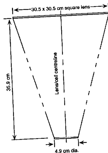
Figure 6.15: Typical arrangement of lens and cell in a photovoltaic concentration system.
