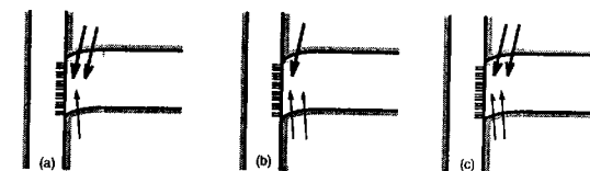
Figure 10.12: Surface recombination resulting from asymmetrical capture cross sections for electrons and holes. The probability of capture depends on both the capture cross section of the interface states and the interface concentrations of the respective carriers. The widths of the arrows represent the probability contribution from the former, while the number of arrows indicates that from the latter. The overall surface recombination rate is determined by the weakest link in terms of the weight of arrows: (a) n-type silicon at low cell voltages, where hole capture is the rate-limiting process; (b) p-type silicon at low cell voltages, where electron capture can be rate limiting; (c) n-type and p-type silicon at high cell voltages, where hole capture is rate limiting.
