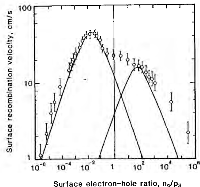
Figure 9.8: Measured effective surface recombination velocity for p-type silicon-oxide interface as a function of surface potential as given by the surface electron/hole ratio ( n_s/p_s ). The bulk injection level was such that n_D was equal to 3 \times 10^{16}/\text{cm}^3 and p_D was equal to 5.5 \times 10^{16}/\text{cm}^3 . The surface recombination velocity is that referred to n_s rather than n_s . The solid lines are theoretical curves for states with two different capture cross-section ratios ( \sigma_n/\sigma_p ) (after Yablonovitch et al. [9.36]).
