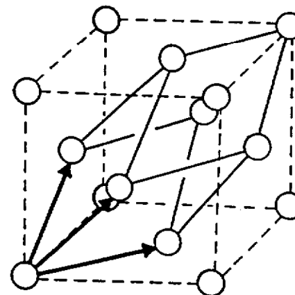
Figure 2.2: The Primitive Cell and the Basis Vectors of the Face-Centred Cubic Space Lattice
