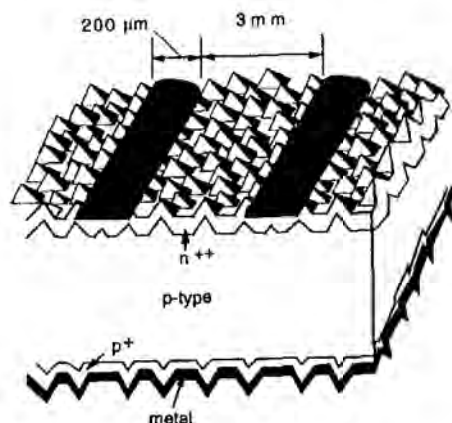
Figure 11.1: Screen printed crystalline silicon solar cell (not to scale).
