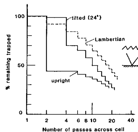
Figure 6.12: Light trapping properties of upright and tilted pyramids (random layout).
