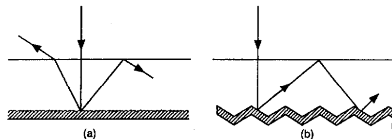
Figure 6.1: Two schemes for trapping light into a solar cell; (a) scheme based upon internal randomization of the light direction; (b) geometrically based scheme.
