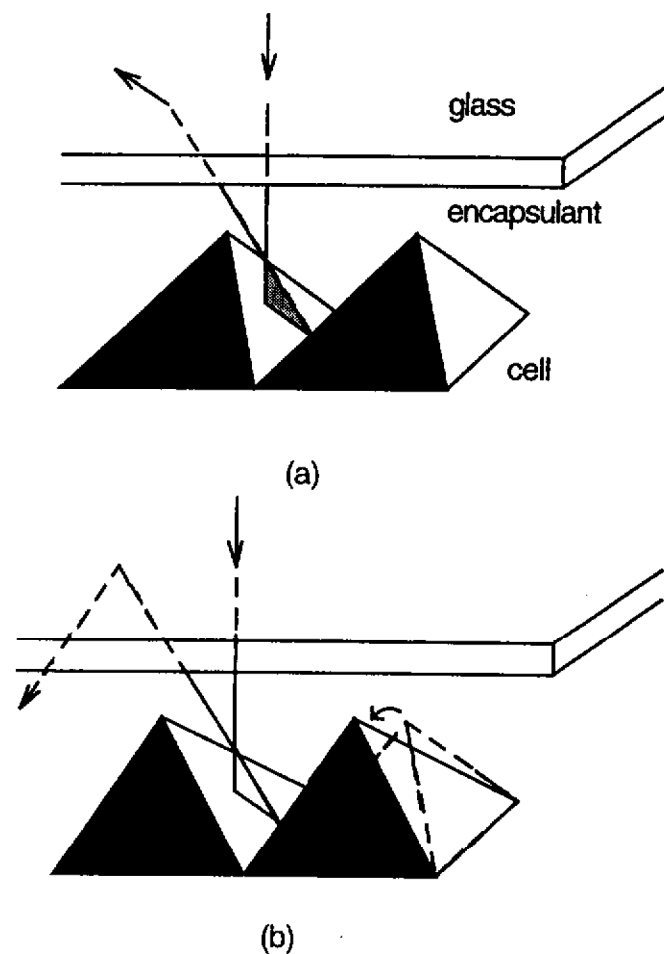
Figure 6.19: Ray paths for pyramidal surface features when encapsulated under glass: (a) normal pyramids; (b) pyramids symmetrically tilted towards one corner.
