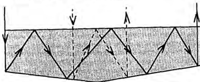
Figure 6.4: Good (solid line) and bad (dashed) ray paths for light trapping with rear surface slats.
