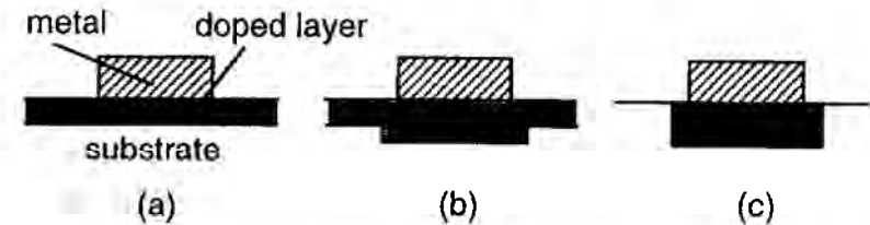
Figure 9.11: (a) Metal contact to a thin doped layer; (b) incorporation of a second, more substantially doped region into the contact area; (c) passivation of contact recombination by a heavily doped region where doped surface layers are not used for surface passivation.
