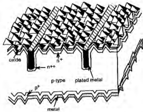
Figure 11.4: Buried contact solar cell.
