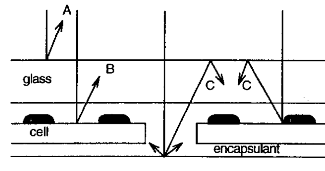
Figure 6.17: Reflections within a typical module.
