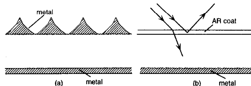
Figure 6.16: Two different schemes for enhancing light trapping for cells where a limited acceptance angle is adequate: (a) use of a secondary surface concentrator; (b) use of an anti-reflection coating with a high degree of angular selectivity.
