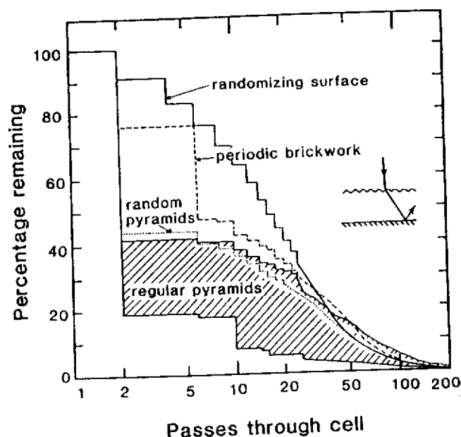
Figure 6.8: Fraction of rays remaining trapped in cell as a function of the number of passes across the cell for cells with top surface structure. The Lambertian case is shown for comparison. The "periodic brickwork" entry corresponds to the "Tilers pattern" of Fig. 6.9.
