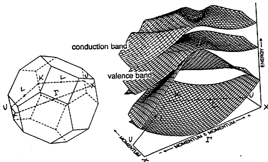
Figure 2.6: (a) Plane of high symmetry within Brillouin zone: (b) E - k relationships for k values lying on this plane.
