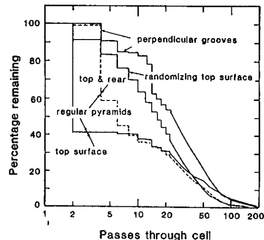
Figure 6.11: Light-trapping properties of double-sided light-trapping schemes involving structure on both cell surfaces. Shown is the fraction of light remaining trapped as a function of the number of passes across the cell.
