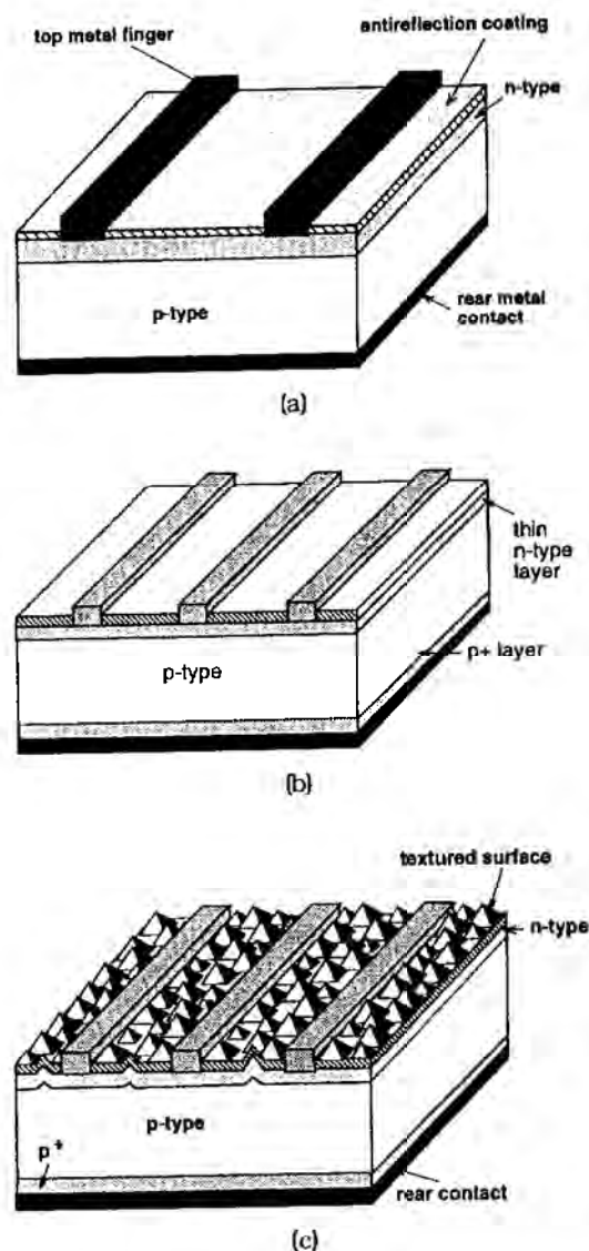
Figure 10.2: (a) Space silicon cell design developed in the early 1960's which became a standard design for over a decade; (b) shallow junction "violet" cell; (c) chemically textured non-reflecting "black" cell.
