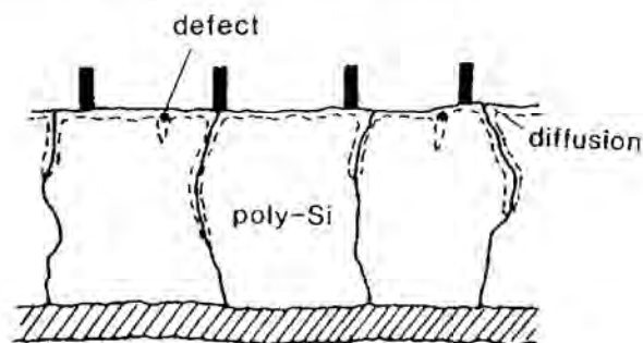
Figure 13.2: Cross-section of a multicrystalline silicon solar cell showing preferential diffusion of dopants down the grain boundaries and at crystallographic defects.
