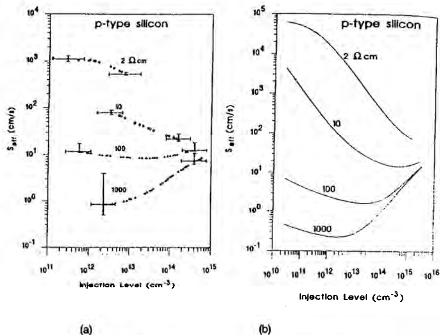
Figure 9.7: (a) Measured surface recombination velocity for oxidized p-type wafers of different resistivity as a function of injection level; (b) corresponding calculated values.
