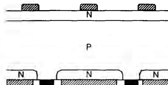
Figure 13.5: Schematic diagram of a double-sided cell structure particularly appropriate to intermediate quality material (carrier diffusion lengths equal to about half the substrate thickness).
