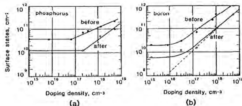
Figure 9.4: Surface state (interface trap) density versus doping level at an oxide passivated surface for (a) phosphorus-doped (n-type) and (b) boron-doped (p-type) surfaces. Results are shown before and after annealing at 450°C (after Snel [9.20]).
