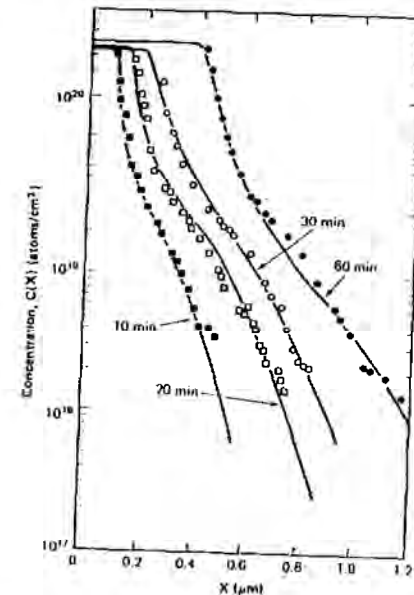
Figure 10.3: Profiles of electrically active phosphorus in silicon as a function of diffusion time at 1000^\circ\text{C} (after Tsai [10.21], © 1969 IEEE).
