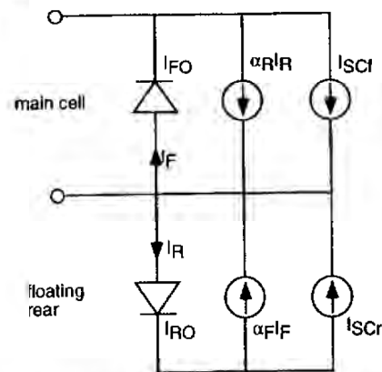
Figure 11.7: Ebers-Moll equivalent circuit for a floating junction solar cell.
