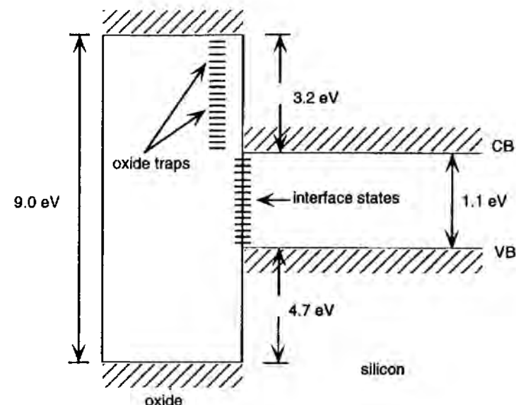
Figure 9.2: The oxide-silicon interface (not to scale; band-bending effects not shown).
