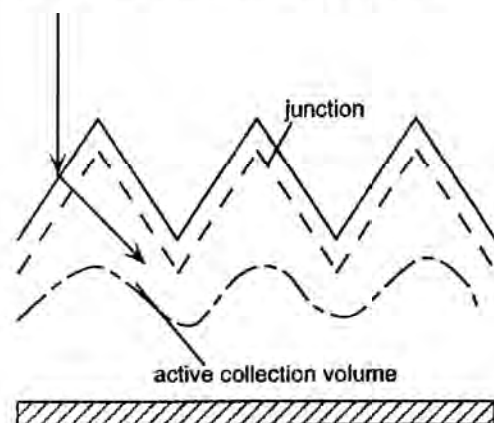
Figure 13.7: Macrogrooved cell structure which combines good reflection properties with the ability to steer light into the active collecting areas of the cell. By choosing an appropriate size for the geometrical features, this approach can significantly boost the performance of even very low quality material [13.18].
