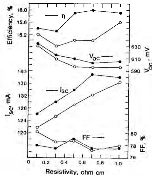
Figure 13.4: Effect of phosphorus pre-treatment upon the performance of cells fabricated on multicrystalline silicon (nominal cell area: 4.06 cm 2 ). The open circles show the results for cells fabricated with a standard PESc sequence, while the closed circles show the benefits of heavy phosphorus diffusion followed by a chemical etch-back [13.20].
