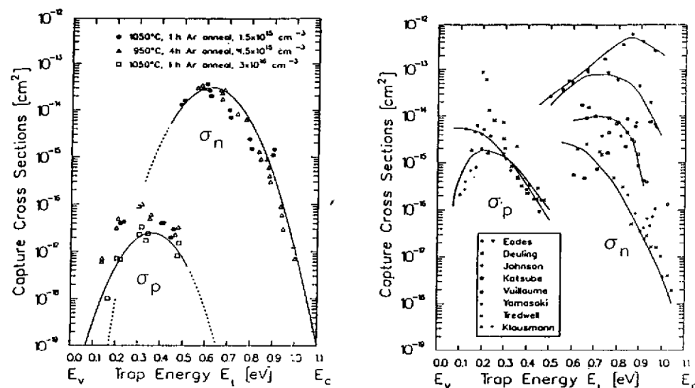
Figure 9.6: (a) Electron and hole capture cross-sections at the Si-SiO 2 interface measured by small pulse DLTS for different oxidation schedules and doping densities; (b) Survey of published data for the electron and hole capture cross-sections at the Si-SiO 2 interface. The solid lines are guides to the eye (Eades [9.27], Deuling [9.28], Johnson [9.29], Katsube [9.30], Vuillaume [9.31], Yamasaki [9.32], Tredwell [9.33], Klausmann [9.34]) (after [9.26]).
