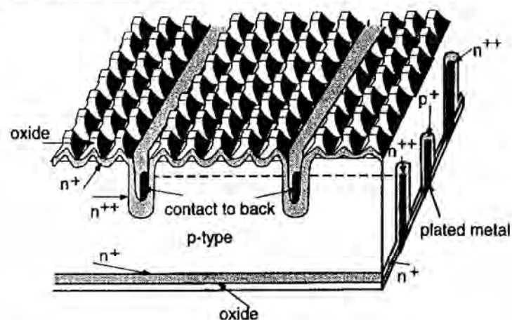
Figure 13.6: Emitter wrap through cell based on the buried contact approach. Both contacts are on the cell rear.
