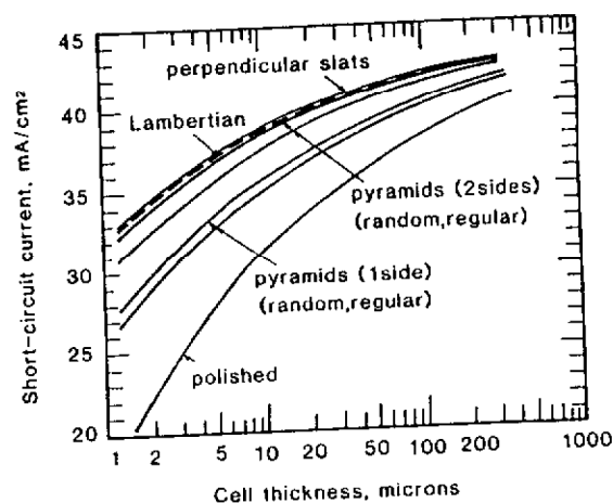
Figure 6.13: Calculated short-circuit current density as a function of silicon cell thickness for various light-trapping schemes (after Campbell & Green [6.13]). All schemes assume zero front surface reflection and a perfect rear reflector. (The illumination used was the global AM1.5 spectrum of Appendix H with a power density of 97 mW/cm 2 ).
