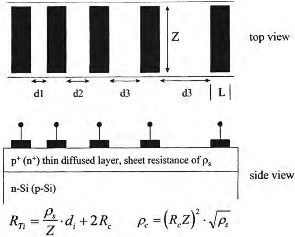
Fig. 2.2. The TLM measurement structure.
