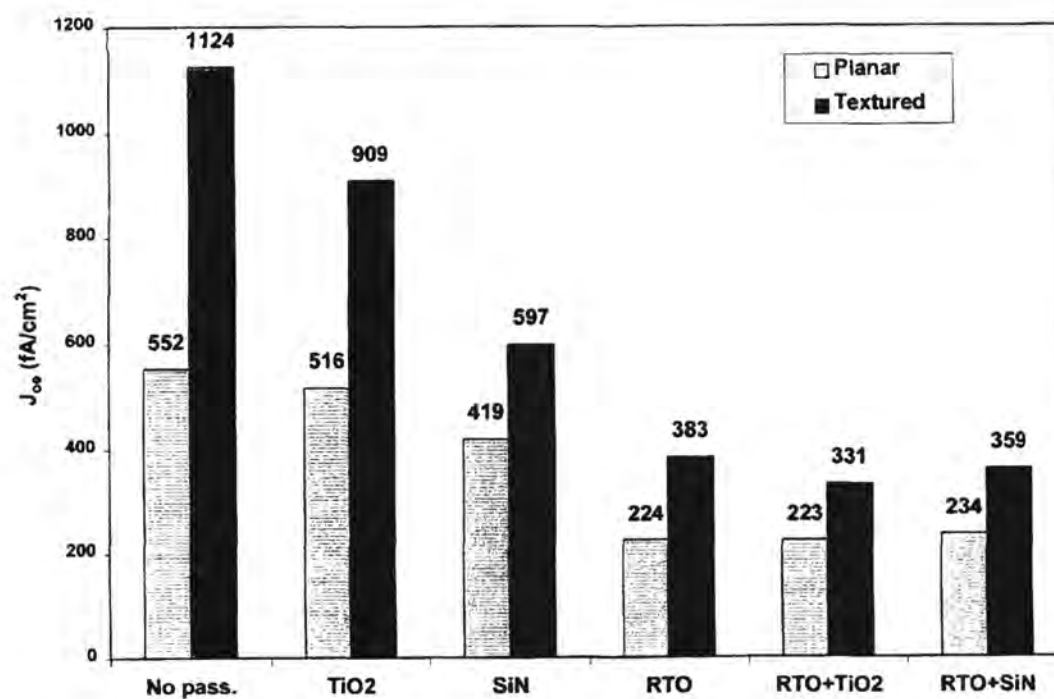
Fig.1.2 Emitter saturation current densities for 40 \Omega/\square RTP emitter.
