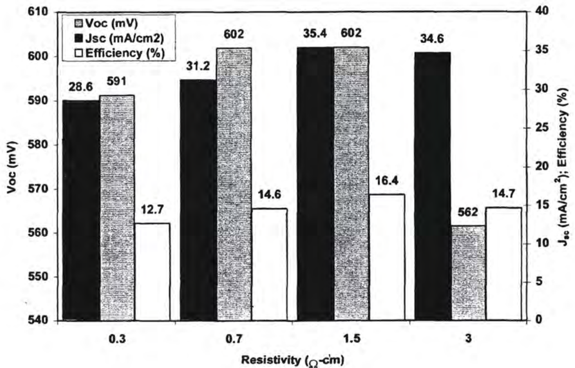
Fig. 7.1: Doping dependence of string ribbon cell efficiency.
