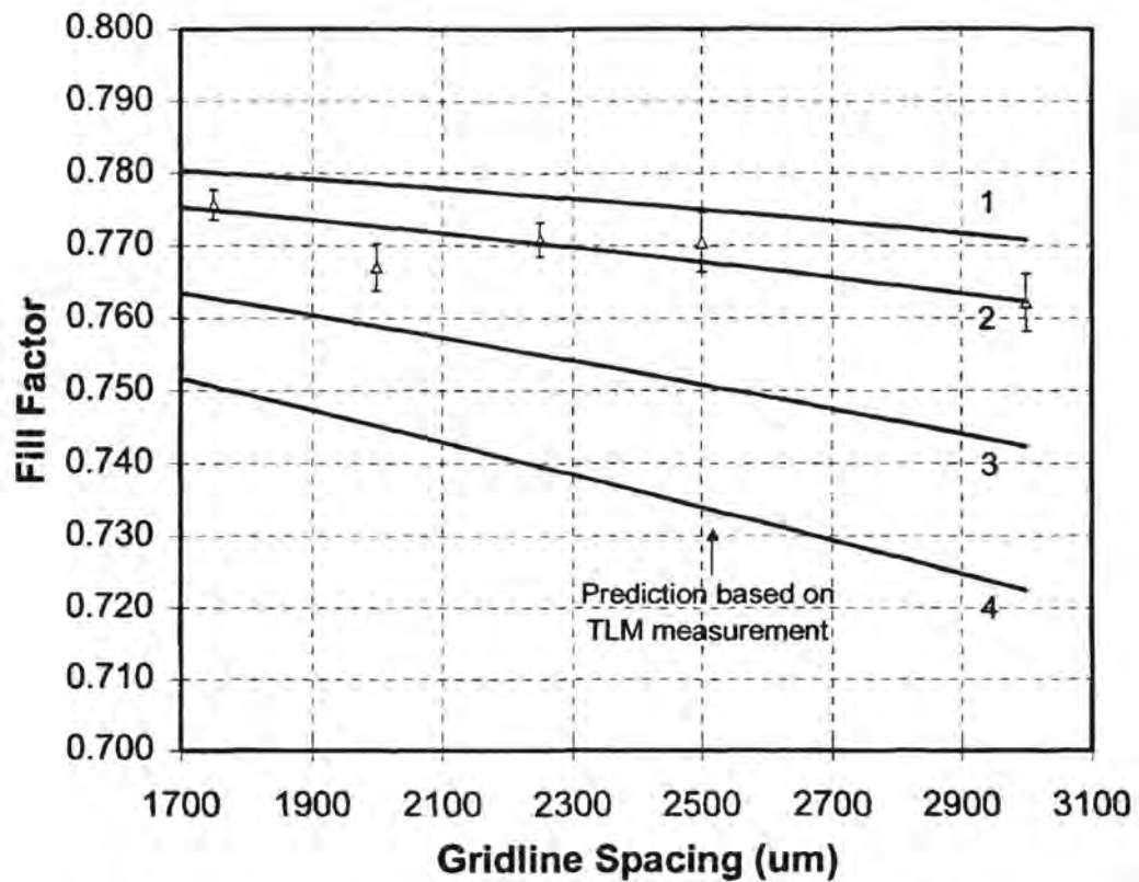
Fig. 2.7. Fill factor versus GBC rear line spacing for 1.3 \text{ }\Omega\text{-cm} substrate material. The solid lines are simulated values for rear \rho_c values of: 1) 1 \text{ m}\Omega\text{-cm}^2 , 2) 10 \text{ m}\Omega\text{-cm}^2 , 3) 30 \text{ m}\Omega\text{-cm}^2 , and 4) 50 \text{ m}\Omega\text{-cm}^2 . The triangles represent experimental data.
