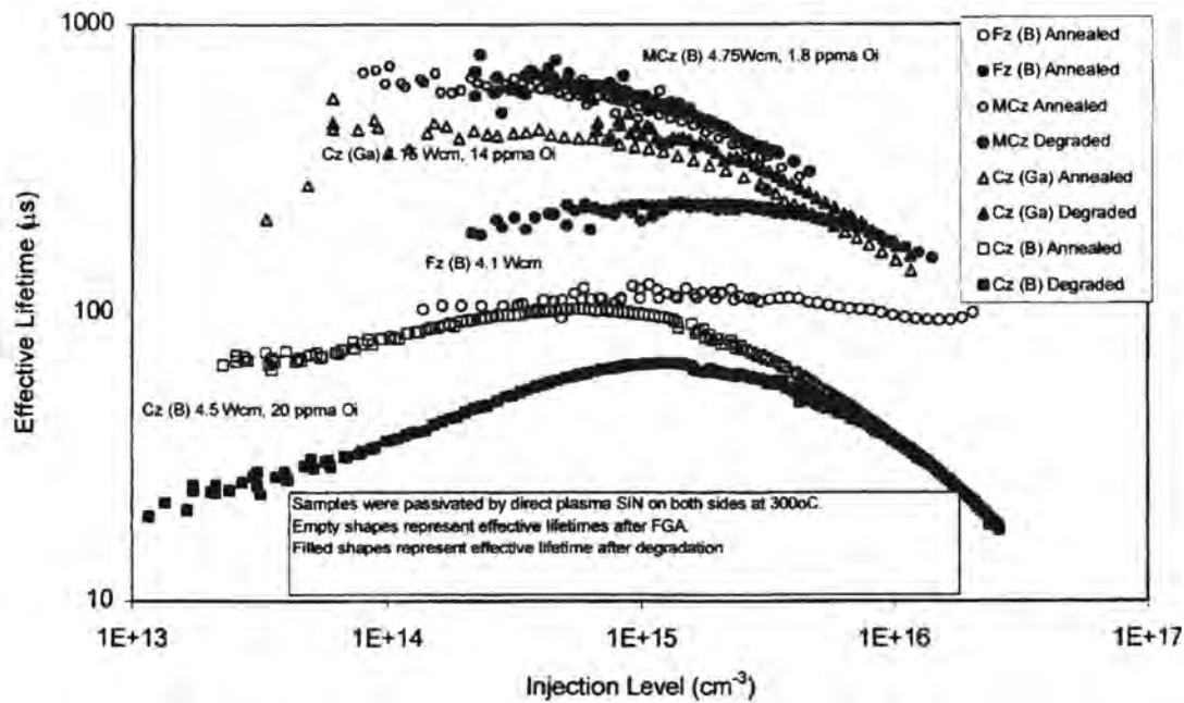
Fig. 3.4: Effective lifetime for 4-5 \Omega -cm samples before and after degradation. Only samples with both high Oi and Bi content showed any degradation.
