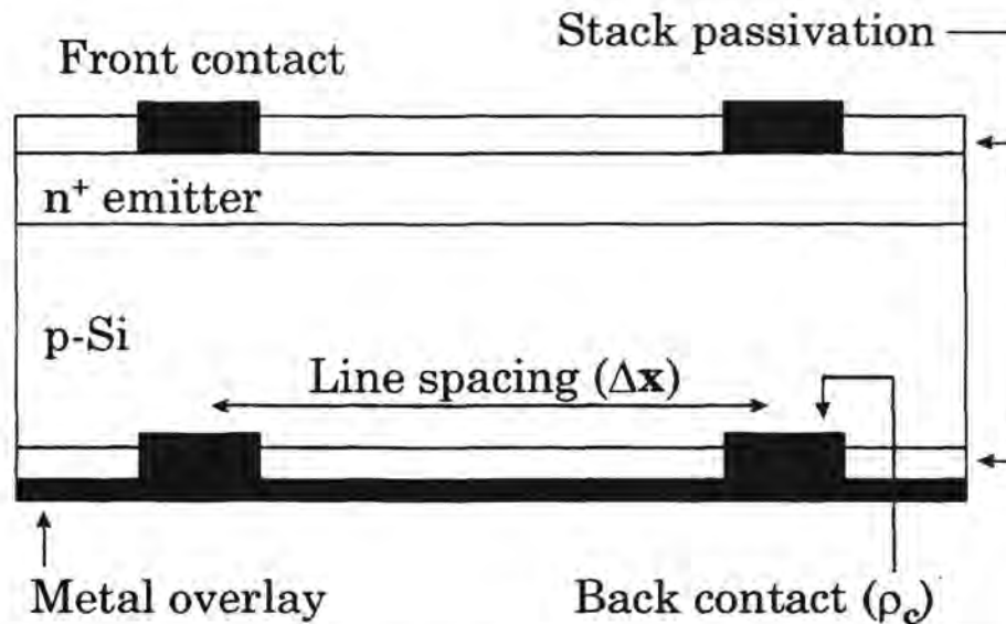
Fig. 2.6. Device structure used to study the effects of \rho_c and x on FF. The effects of P_{finger} and P_{bus} for the rear electrode were removed by the metal overlay.
