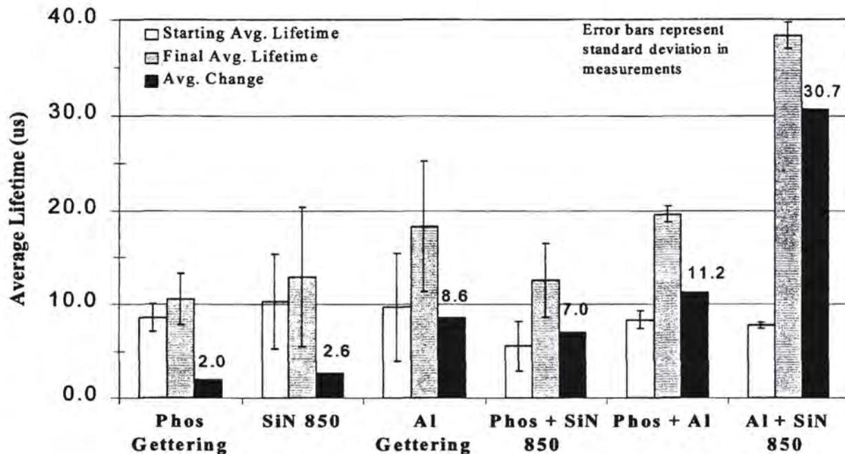
Figure 1.9 Effectiveness of gettering and passivation treatments
