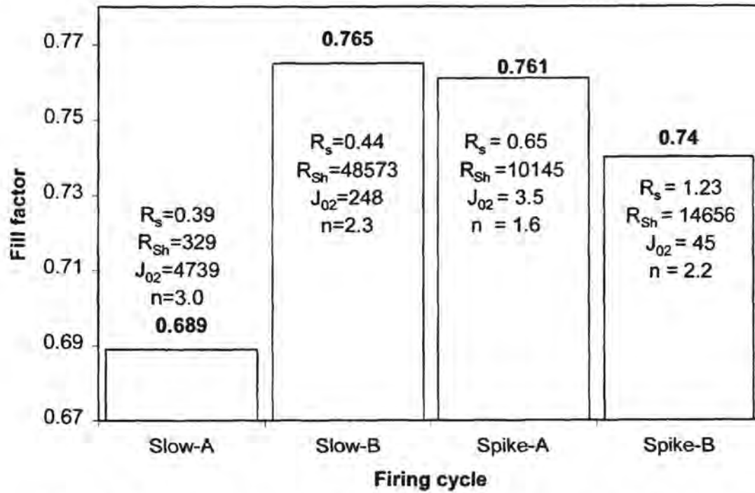
Fig. 5.3: Effect of paste and firing cycle on fill factor of screen-printed solar cells on mc-Si with 0.25 \mu\text{m} deep emitter.
