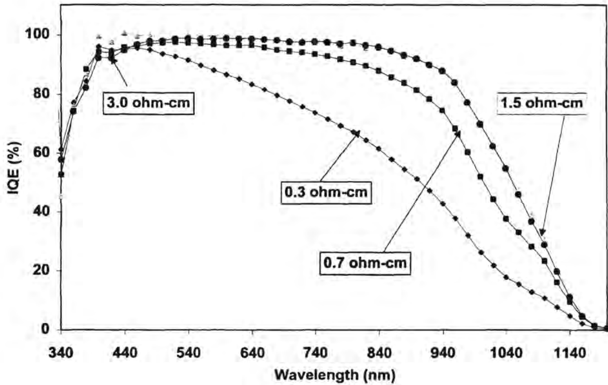
Fig. 7.2: Resistivity effect on string ribbon IQE.
