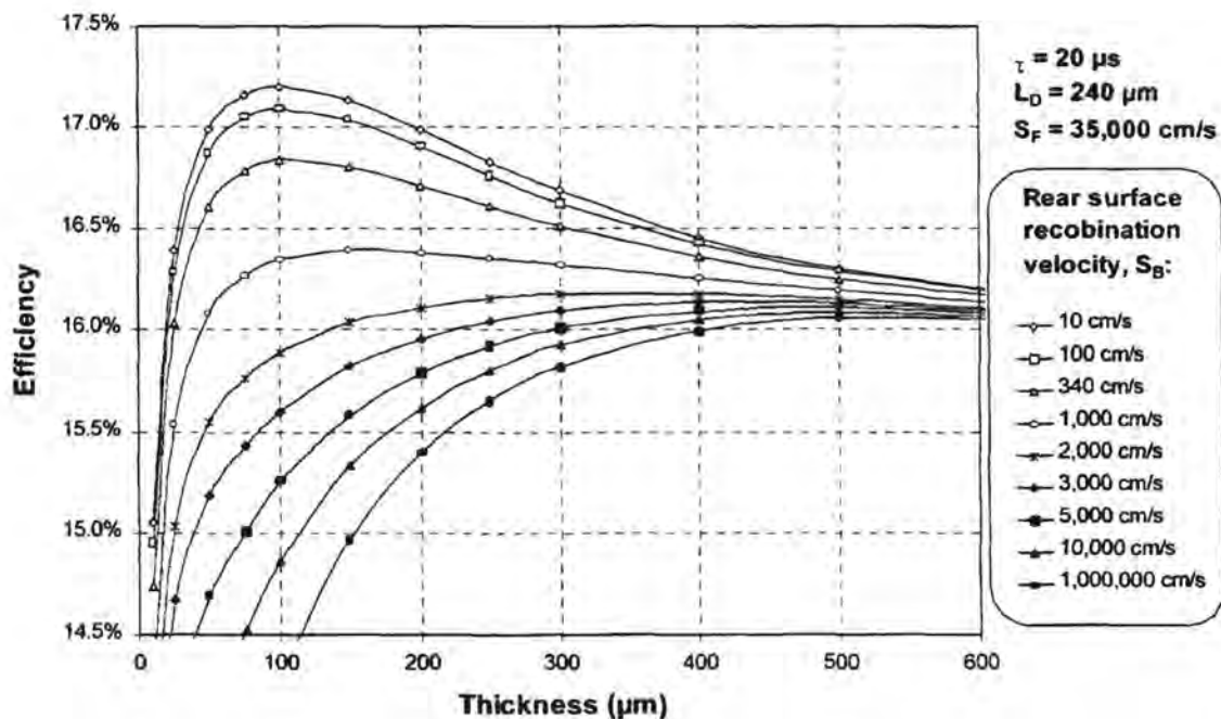
Fig. 1.1 Effect of rear passivation on optimum solar cell thickness.
