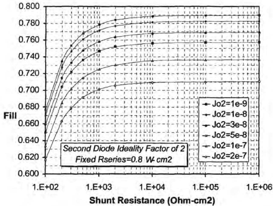
Fig. 5.1: The effect of R_{sh} and J_{02} on FF for 4 \text{ cm}^2 cells
