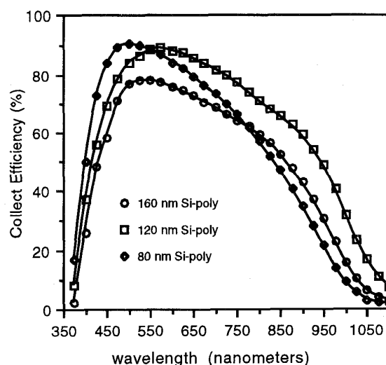
Figure 3: spectral photoresponses of unannealed RT-LPCVD poly-emitter silicon solar cells.
