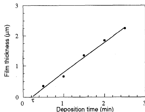
Figure 2: Polysilicon films thickness vs. deposition time. 750 °C, 5 mbar, 10 % SiH 4 in Ar, 50 sccm.
