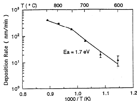
Figure 1: RT-LPCVD deposition rates as a function of the deposition temperature. 1 mbar, 10 % SiH 4 in Ar, 100 sccm.
