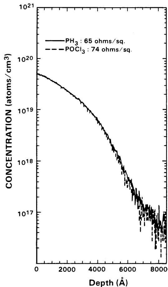
Figure 1. Doping profiles obtained by SIMS measurements for two wafers after the drive-in diffusions. The surface concentration and depth-dependence for the two doping sources are very similar.
