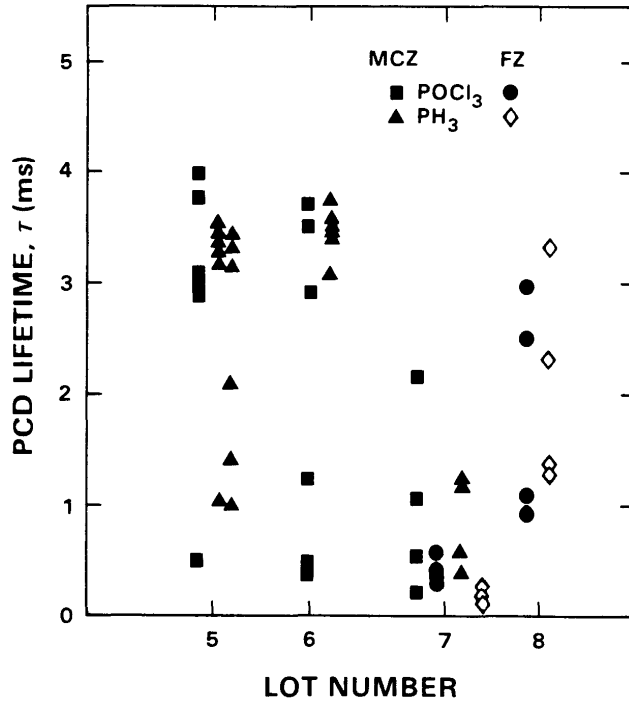
Figure 3. PCD lifetime of wafers after diffusion for several lots for both doping sources and two wafer material types (MCZ and FZ). The accuracy of the measurement is \pm 5\% .
