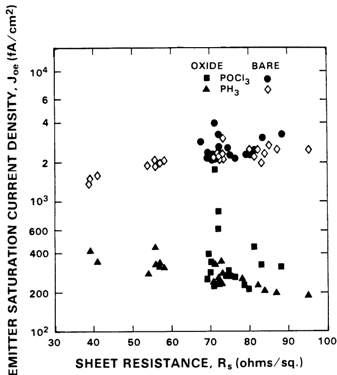
Figure 2. Dependence of J_{oe} on R_s for both doping sources for oxide-passivated and bare wafers. The uncertainty in the measurement is \pm 10\% .
