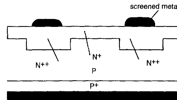
Figure 11.3: Ideal situation for fine linewidth screen printed metallization with contact being made to selectively doped areas.
