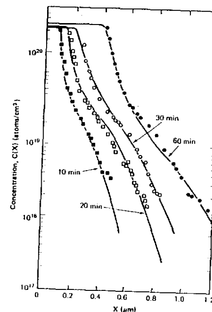
Figure 10.3: Profiles of electrically active phosphorus in silicon as a function of diffusion time at 1000^\circ\text{C} (after Tsai [10.21], © 1969 IEEE).
