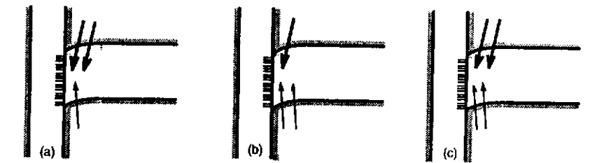
Figure 10.12: Surface recombination resulting from asymmetrical capture cross sections for electrons and holes. The probability of capture depends on both the capture cross section of the interface states and the interface concentrations of the respective carriers. The widths of the arrows represent the probability contribution from the former, while the number of arrows indicates that from the latter. The overall surface recombination rate is determined by the weakest link in terms of the weight of arrows: (a) n-type silicon at low cell voltages, where hole capture is the rate-limiting process; (b) p-type silicon at low cell voltages, where electron capture can be rate limiting; (c) n-type and p-type silicon at high cell voltages, where hole capture is rate limiting.
