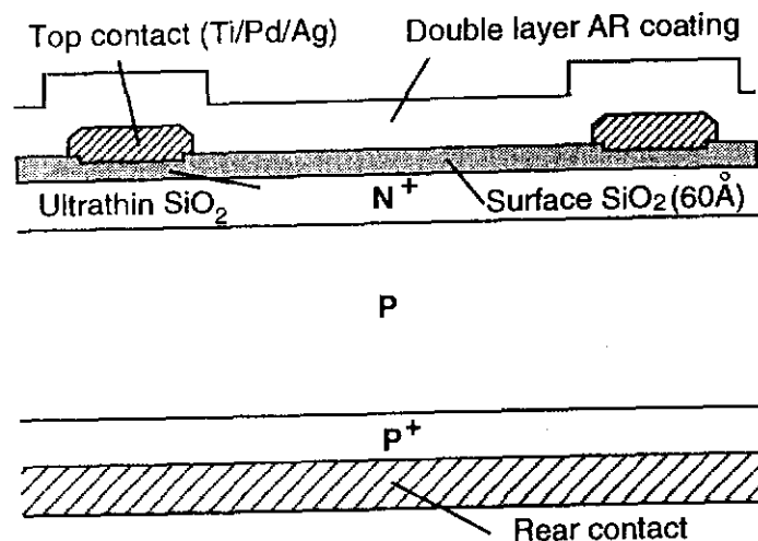
Figure 10.6: Metal-Insulator-NP junction (MINP) solar cell.
