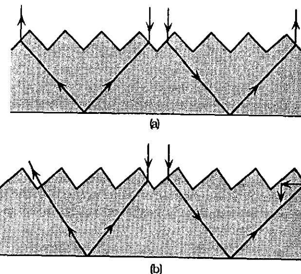
Figure 6.5: Light-trapping with top surface grooves formed by intersecting (111) equivalent planes: (a) untilted structure; (b) effect of a slight tilt.
