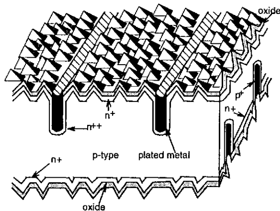
Figure 11.6: Double-sided or bifacial buried contact solar cell.
