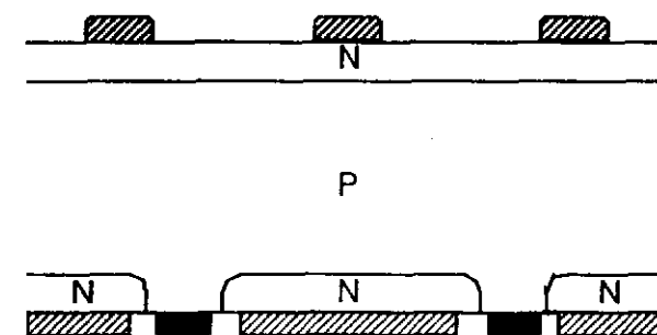
Figure 13.5: Schematic diagram of a double-sided cell structure particularly appropriate to intermediate quality material (carrier diffusion lengths equal to about half the substrate thickness).
