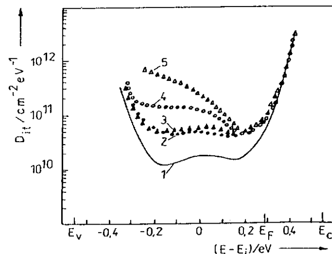
Figure 9.3: Degradation of the interface state density of Al/SiO 2 /Si and SiO 2 /Si structures by annealing treatments in forming gas (450°C, 30 min.) and dry N 2 (500°C, 5 min). The specimens (thermally oxidized n-Si(111), 10 Ωcm) were well stabilized by a PMA process before initial measurement (curve 1). Al/SiO 2 /Si - annealed in FG (curve 2); annealed in N 2 (curve 3); SiO 2 /Si - annealed in FG (curve 4); annealed in N 2 (curve 5).
