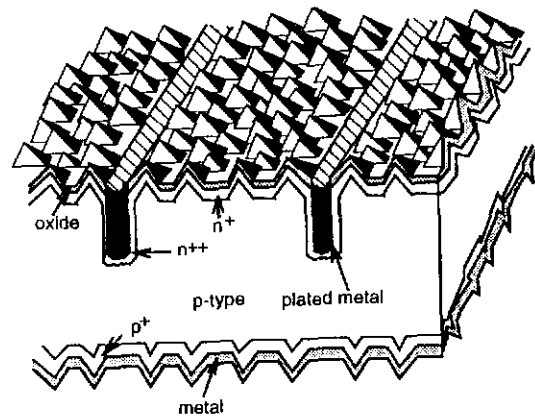
Figure 11.4: Buried contact solar cell.
