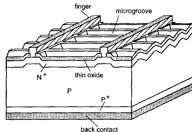
Figure 10.8: The microgrooved PESC cell, the first silicon cell to exceed 20% efficiency in 1985.
