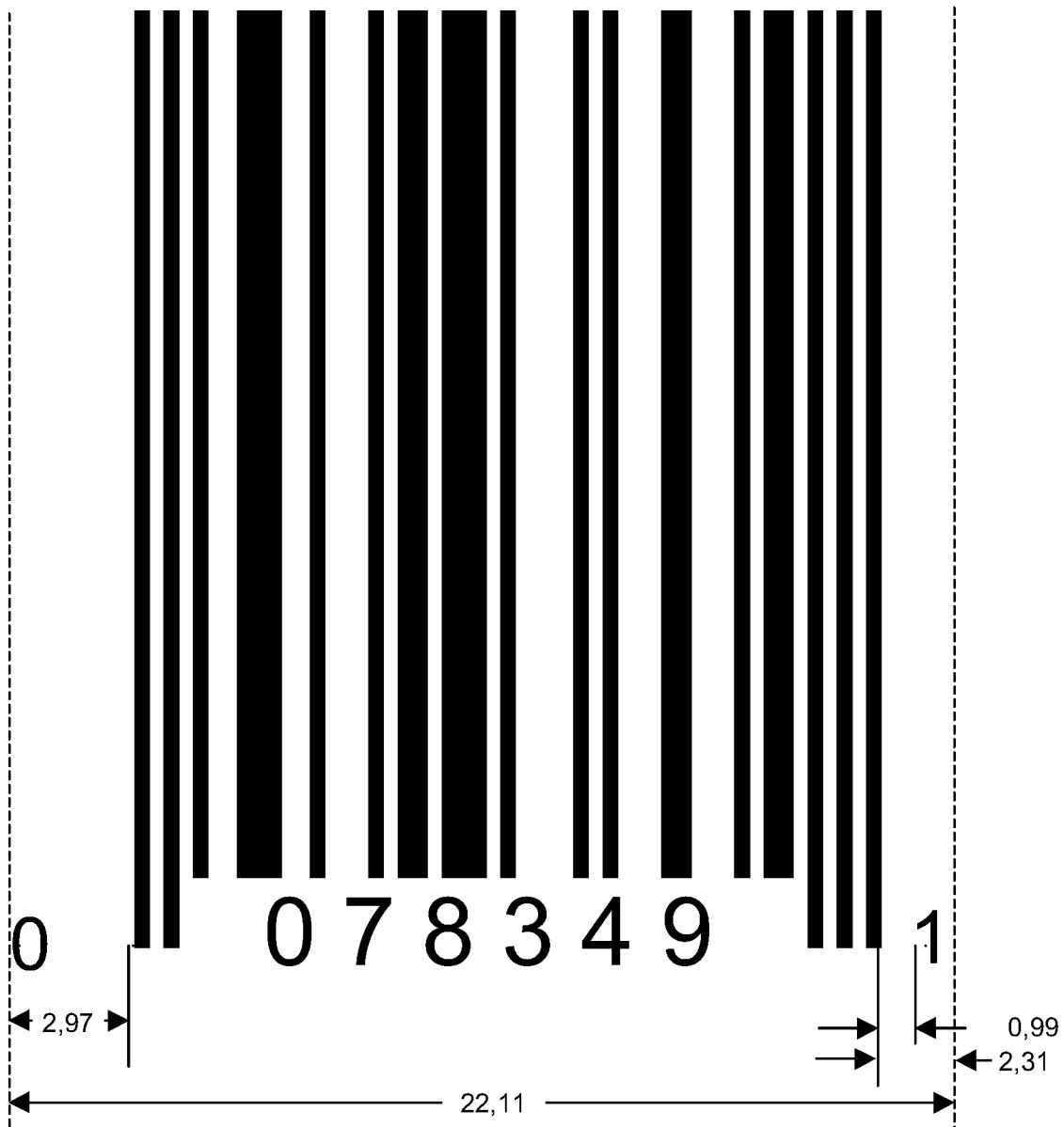
Figure E.5: UPC-E
