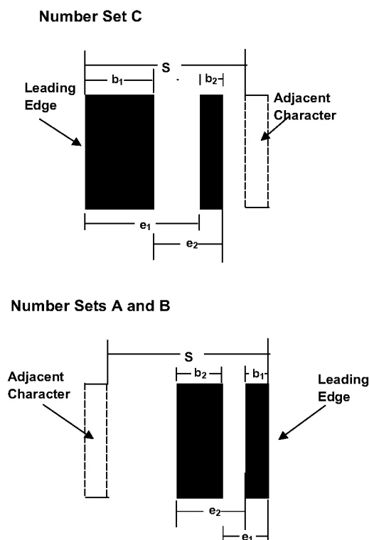
Figure 7: Symbol character decode measurements
