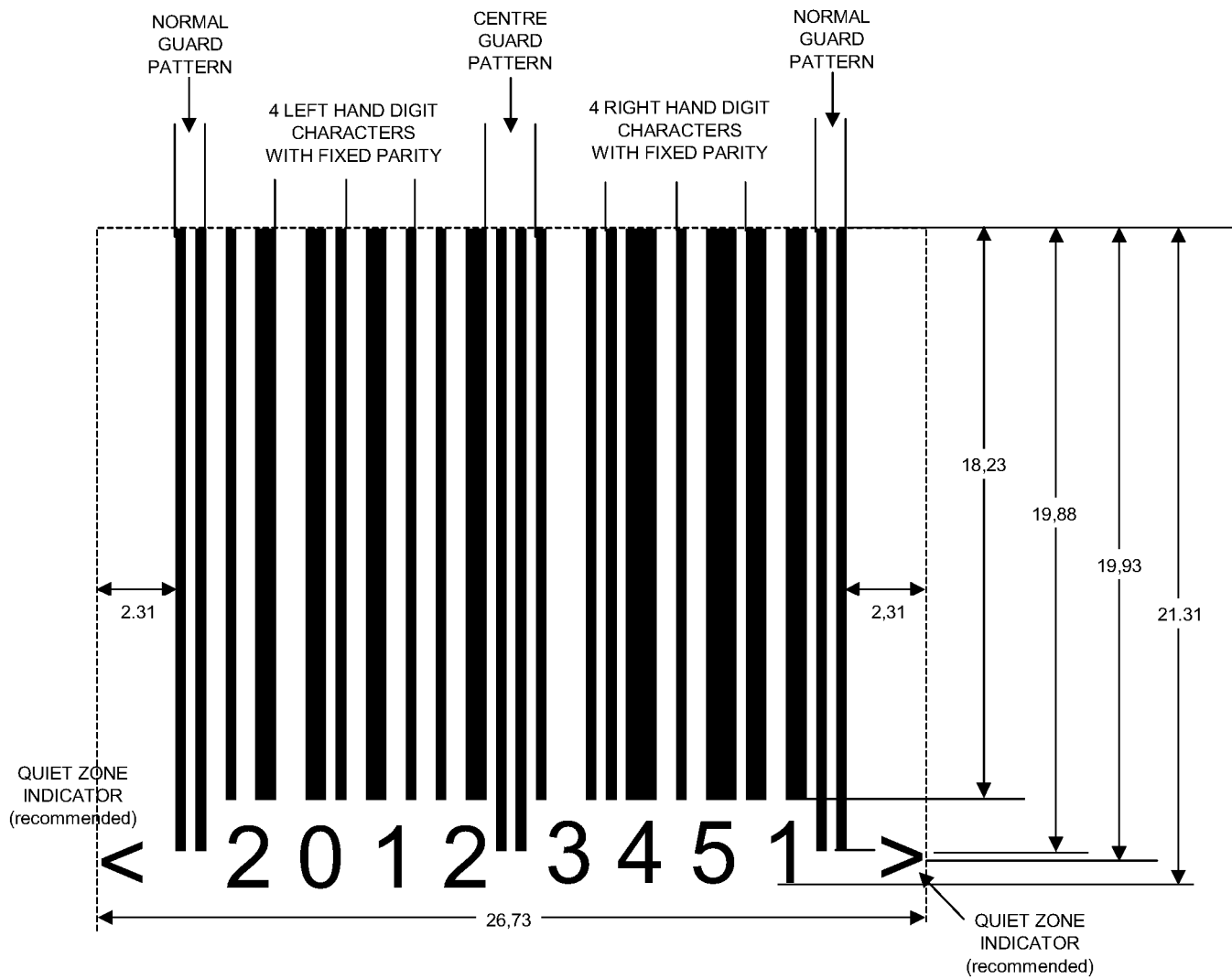
Figure E.4: EAN-8
