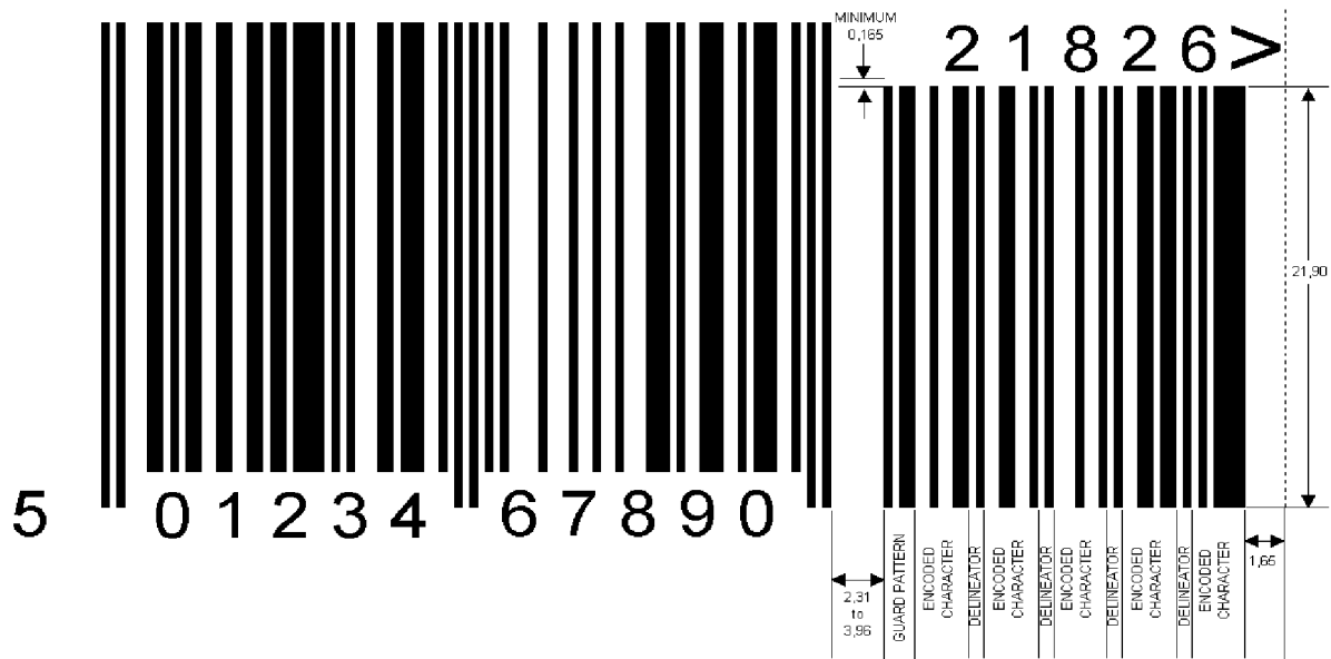
Figure E.7: EAN -13 with 5-digit add-on
