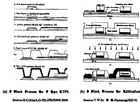
Fig.4 Mask Step Reduction for LTPS Fabrication
