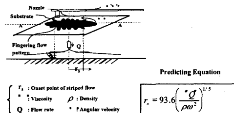
Fig.9 Predicting Equation of Onset Point of Fingering Flow Pattern
