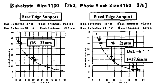
Fig.7 Deflection analysis of photo-mask
