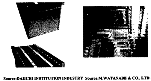
Fig.11 Air Levitation Conveyor System for TFT
