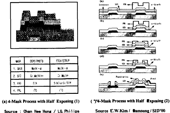
Fig.5 4-Mask Step Process for a-Si Fabrication
