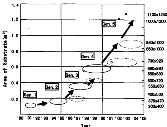
Fig.3 Trend of Substrate Size Expansion
