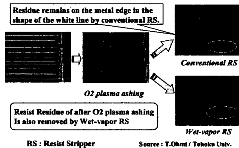
Fig.10 Residue Remove by Wet-vapor RS
