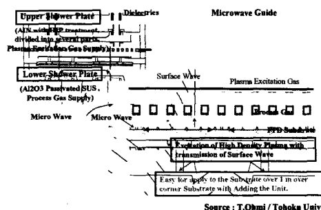
Fig.8 Microwave-Excitation System with RLSA
