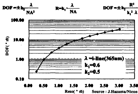
Fig.6 Relation between DOF and Resolution
