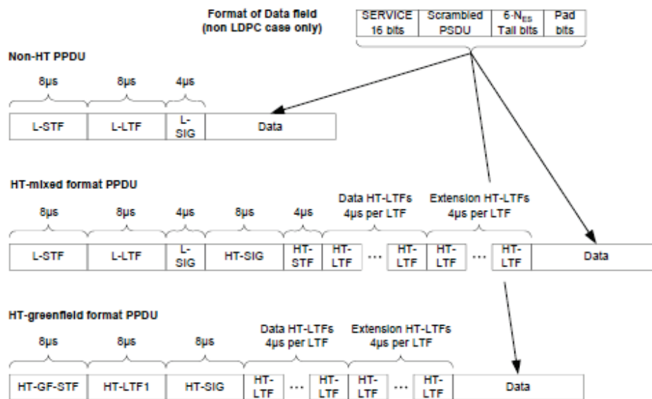
Figure 20-1—PPDU format
