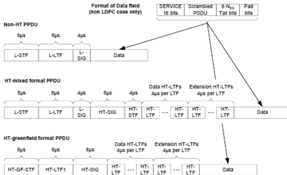
Figure 20-1—PPDU format
