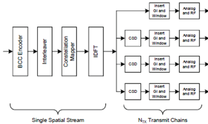
Figure 20-2—Transmitter block diagram 1
