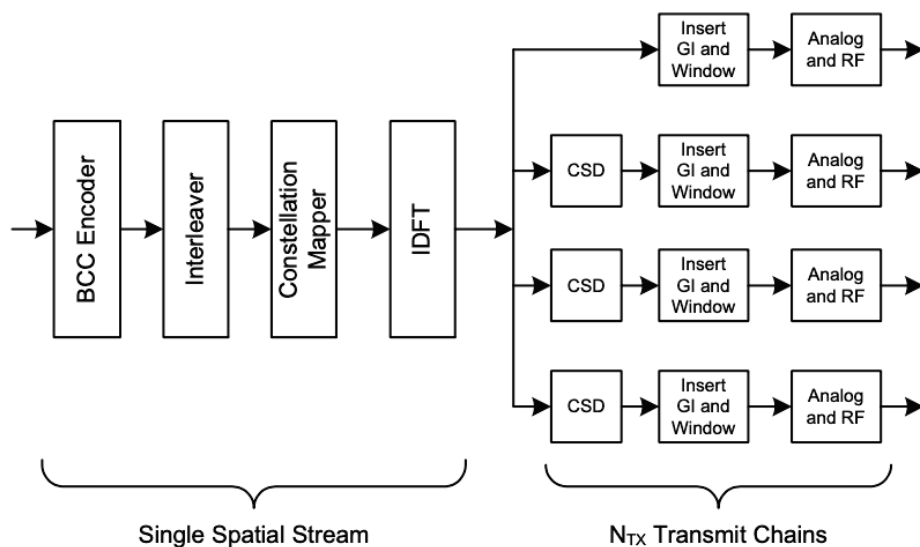
Figure 20-2—Transmitter block diagram 1
