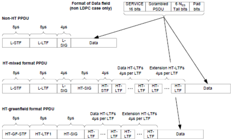
Figure 20-1—PPDU format
