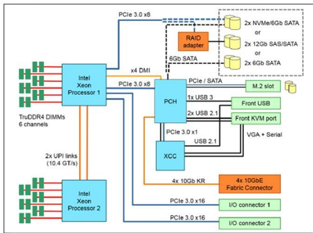
Figure 4. SN550 system architectural block diagram
