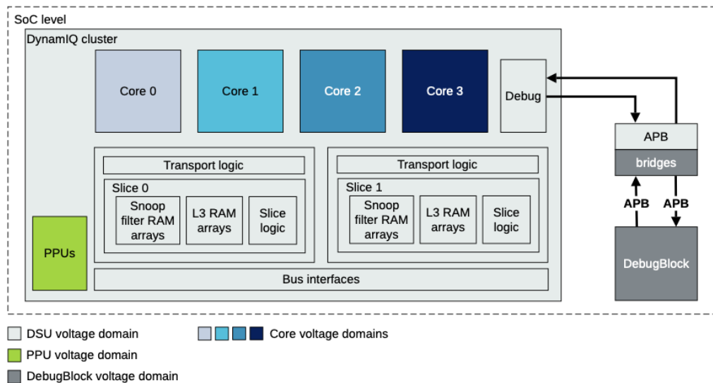
Figure 5-6: DSU-110 voltage domains
