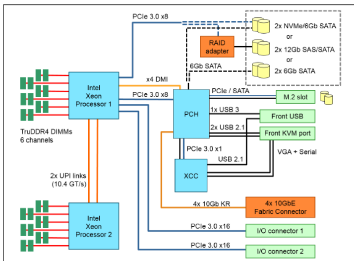
Figure 4. SN550 system architectural block diagram
