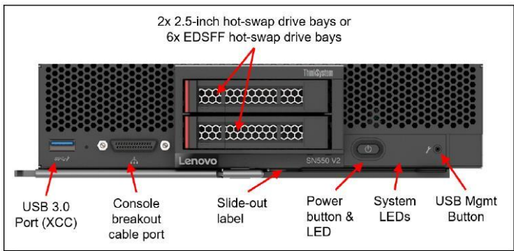
(/assets/images/LP1397/SN550%20V2%20front%20view%20with%20callouts.png) Figure 2. Front view of the ThinkSystem SN550 V2 server
