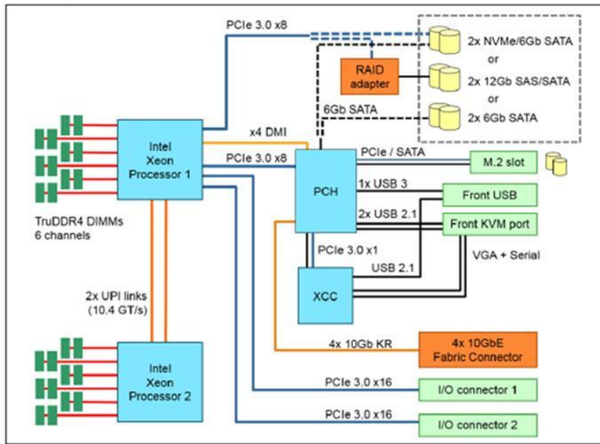
Figure 4. SN550 system architectural block diagram
