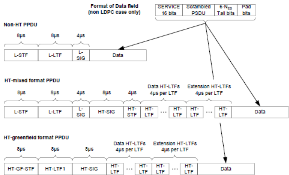
Figure 20-1—PPDU format
