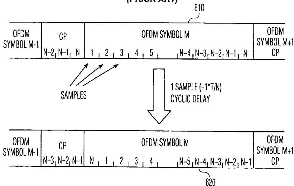
FIG. 7 (PRIOR ART)
