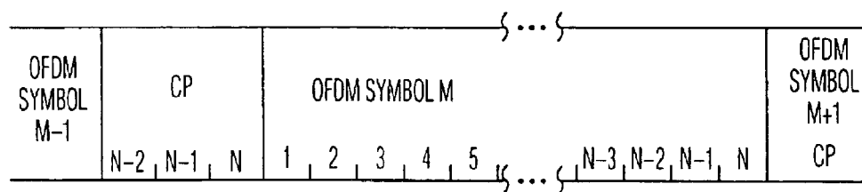
FIG. 2 (PRIOR ART)
