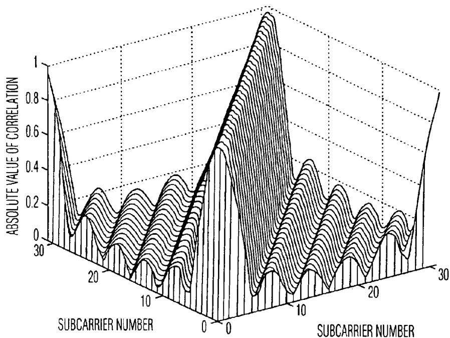
FIG. 7 (PRIOR ART)
