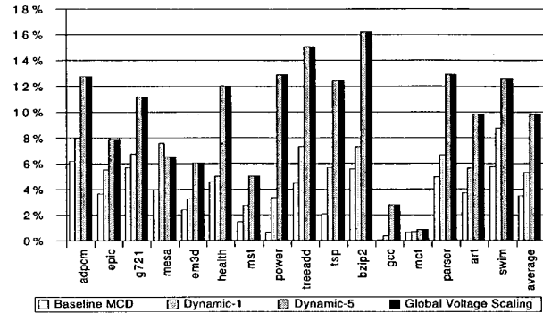
Figure 5. Performance degradation results
