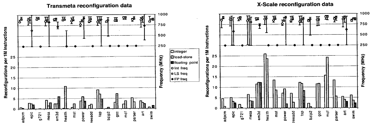
Figure 9. Summary statistics for intervals chosen by the off-line tool for the dynamic 5% configuration . Solid bars indicate, for the integer, load-store, and floating-point domains, the number of reconfigurations requested per 1 million instructions. Points above the bars indicate the average frequencies chosen for those domains. "Error bars", where shown, indicate the range of dynamic frequencies for the domain.
