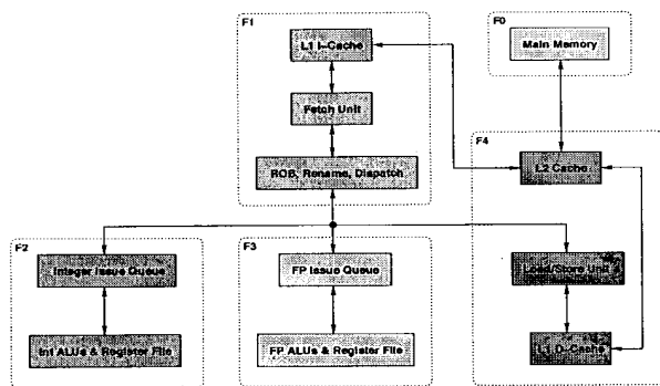
Figure 1. Multiple clock domain processor block diagram
