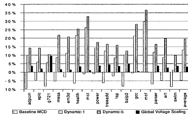
Figure 7. Energy-delay improvement results
