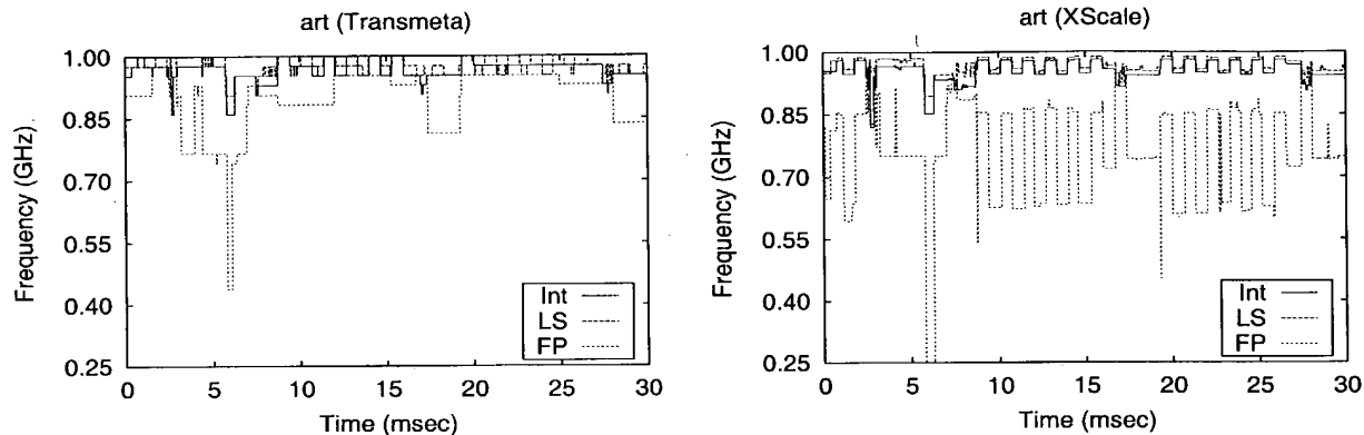
Figure 8. Frequency changes for art generated by our off-line algorithm for the dynamic 1% configuration.
