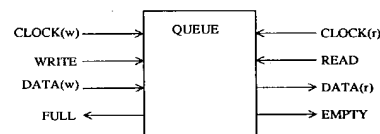
Figure 2. Queue structure
