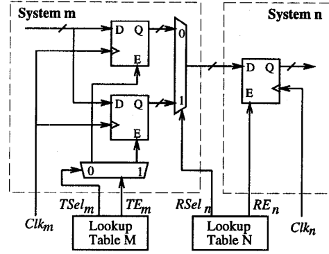
Figure 7: Double-buffered hardware.
