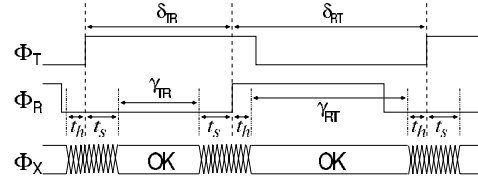
Figure 3. Clock Timing for the FIFO
