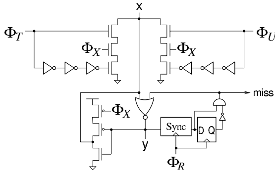
Figure 8. A Miss Detector
