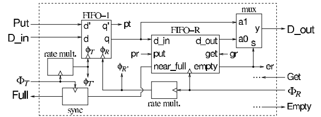
Figure 9. Implementing a FIFO Interface. (See eq. 7 for definitions of Empty, gr, pr)
