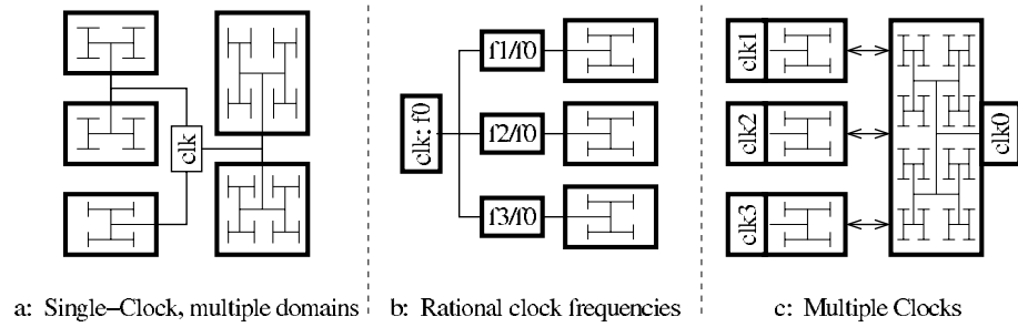
Figure 1. Chips with Multiple Clock Domains
