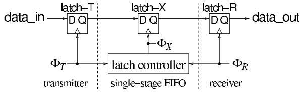
Figure 2. The Single Stage FIFO
