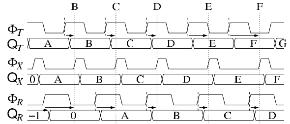
Figure 5. Drifting Skew
