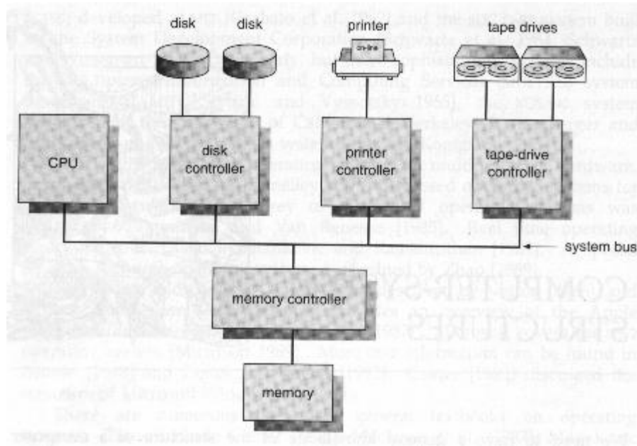
A modern computer system.
