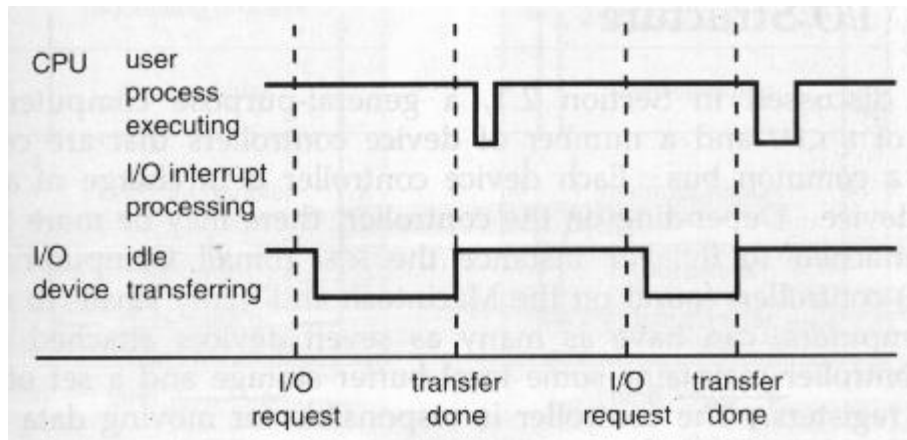
Interrupt time line for a single process doing output.
