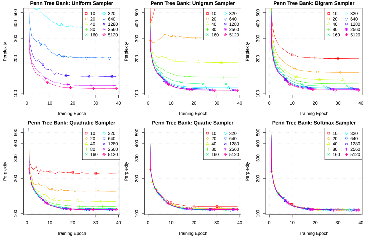
Figure 5. Convergence speed of different sampling distributions ( uniform, unigram, bigram, quadratic, quartic, softmax ) for a varying sample size m \in \{10, 20, 40, \dots\} on the Penn Tree Bank dataset. Once enough samples are taken to remove the bias, adding more samples does not increase convergence speed considerably.
