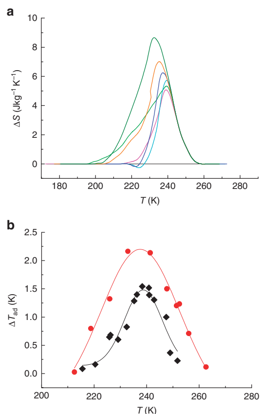
Figure 3 | Barocaloric effects in \text{LaFe}_{11.33}\text{Co}_{0.47}\text{Si}_{1.2} . (a) Isothermal entropy change as a function of temperature associated with the isothermal application of selected hydrostatic pressures. Black lines correspond to 0 kbar; green, 0.8 kbar; magenta, 1 kbar; cyan, 1.2 kbar; blue, 1.4 kbar; orange, 1.7 kbar and olive, 2.1 kbar. (b) Adiabatic temperature change on fast release of hydrostatic pressure. Diamonds correspond to 1 kbar and circles to 2 kbar (lines are guides to the eye).
