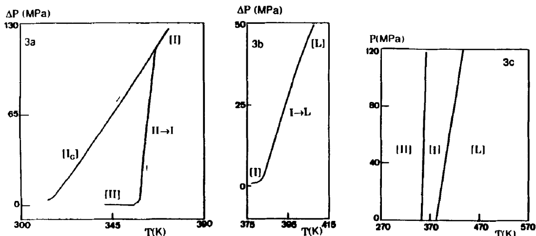
FIGURE 3 Experimental thermobarograms for AMP, n_2 = 2 , (\text{NH}_2)(\text{CH}_3)\text{C}(\text{CH}_2\text{OH})_2 on heating (solid II to plastic I phase transition) and cooling (the reversible transition is absent in the range of temperature studied) (a) and the plastic I to liquid L process (b) and Pressure-Temperature phase diagram (c).
