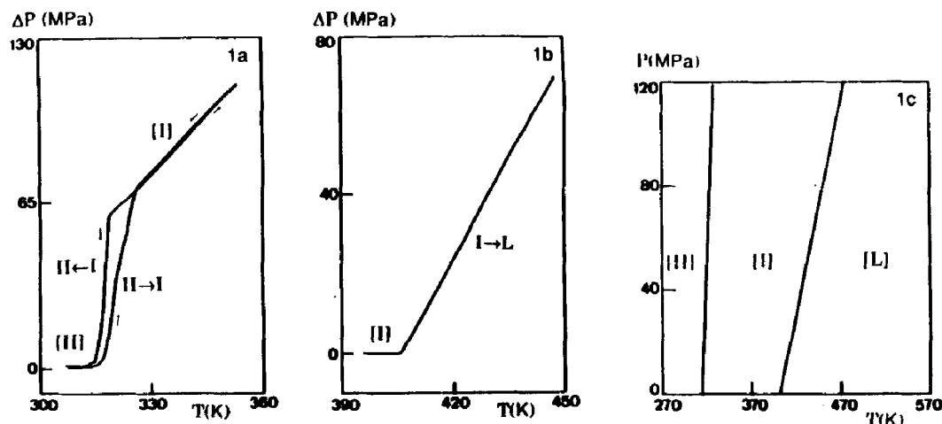
FIGURE 1 Experimental thermobarograms showing for NPG, n_1 = 2 , (\text{CH}_3)_2\text{C}(\text{CH}_2\text{OH})_2 the solid II to plastic I phase transition (on heating and cooling (a)) and the plastic I to liquid L process (b) and Pressure-Temperature phase diagram (c).
