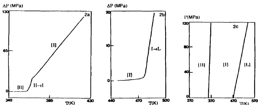
FIGURE 2 Experimental thermobarograms showing for PG, n_1 = 3 , (\text{CH}_3)\text{C}(\text{CH}_2\text{OH})_3 the solid II to plastic I phase transition (a) and the plastic I to liquid L process (b) and Pressure-Temperature phase diagram (c).
