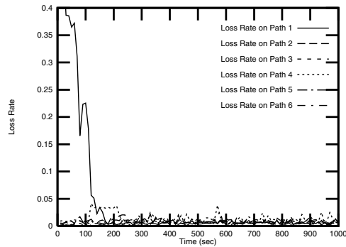
Fig. 8. Loss under DAR traffic for network topology 1
