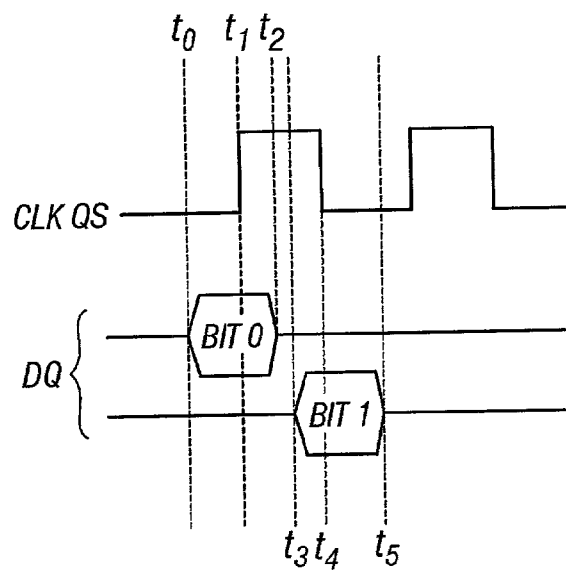
FIGURE 2 (Prior Art)
