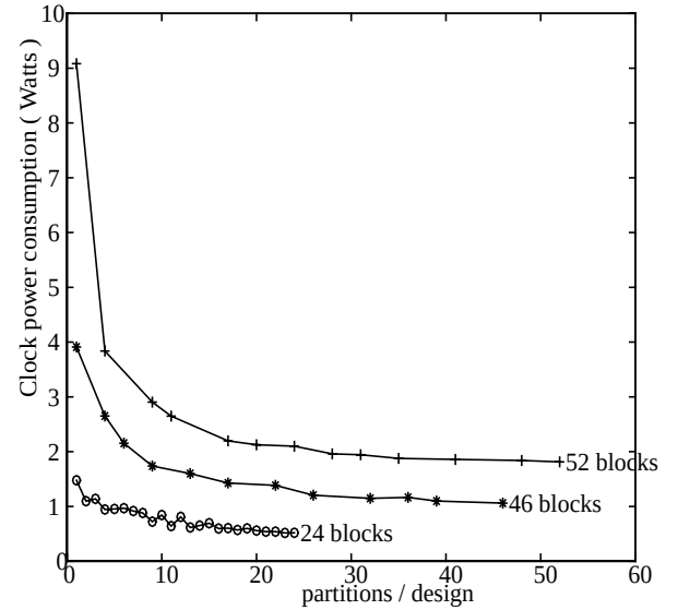
Fig. 4. Power consumption in Clock as a function of partitioning.
