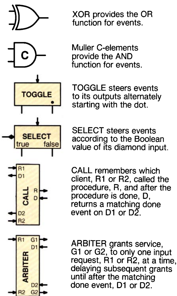
FIGURE 9. Logic Modules for Events
