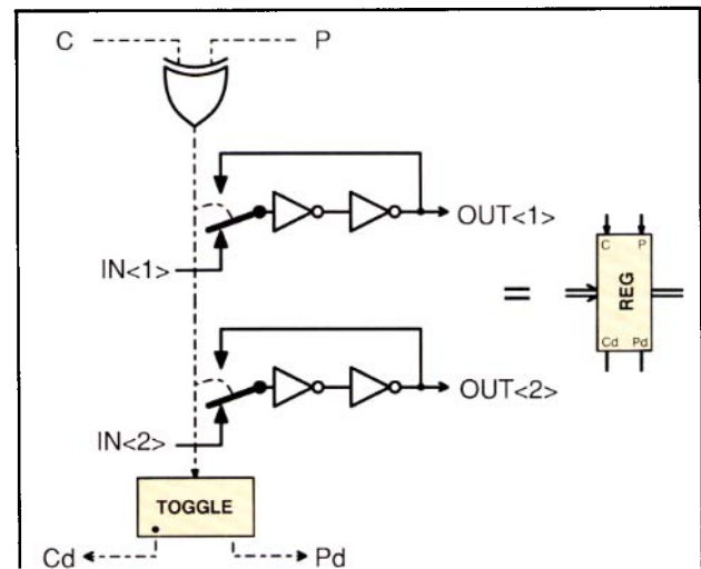
FIGURE 14. Latches Used as an Event-Controlled Storage Register
