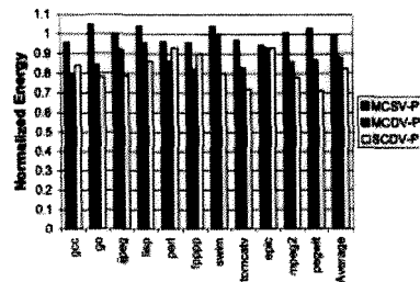
Figure 7. Normalized energy (FIFOs with pauseable clocks)
