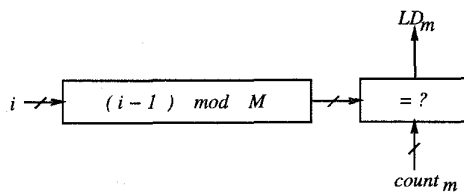
Figure 11: The LD Gen module (of system m ).
