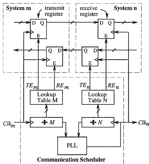
Figure 1: Interface hardware for rational clocking.
