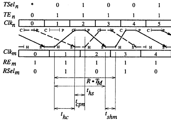
Figure 6: Computing R in the slower receiver case.
