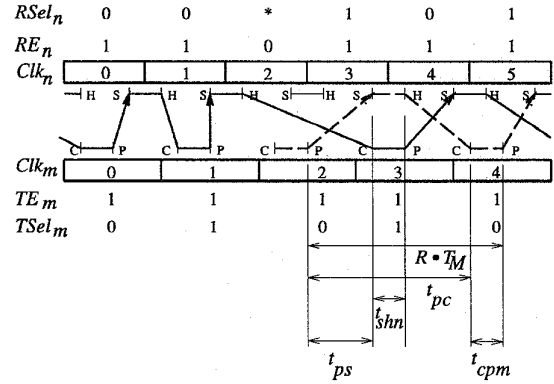
Figure 5: Computing R in the slower transmitter case.
