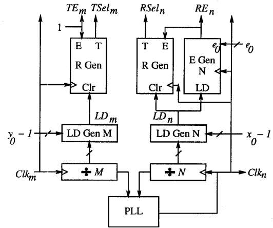
Figure 9: Run-time scheduler for double-buffering. (Only one direction shown.)
