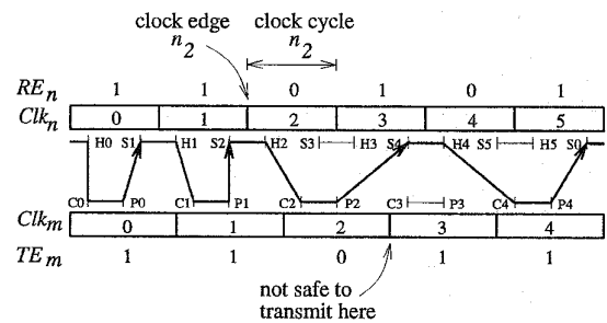
Figure 2: A schedule diagram.
