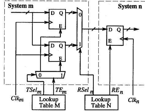
Figure 7: Double-buffered hardware.
