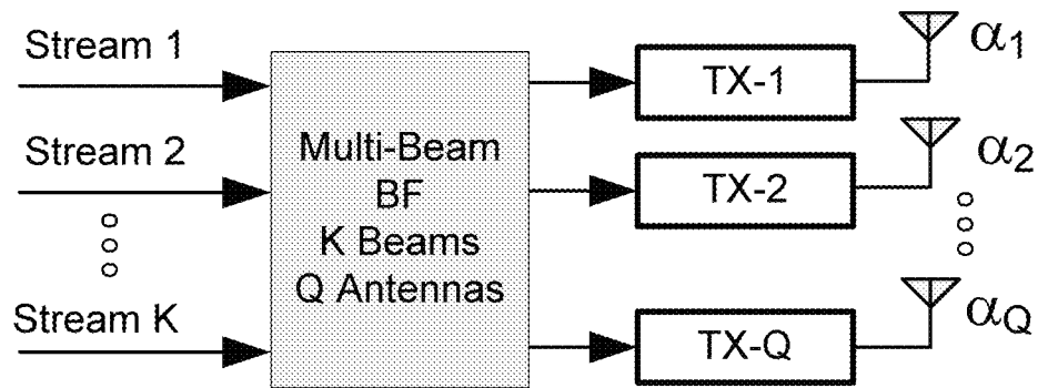
(a) Digital beamforming
