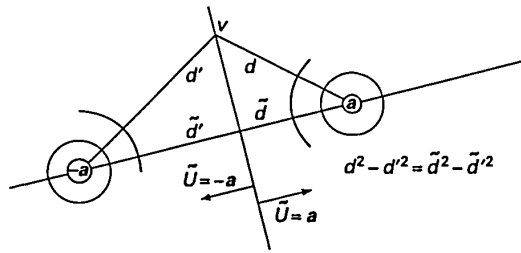
Figure 8.4. ML decision regions for binary signals in WGN. A vector v on the threshold boundary is shown. The distance from v to a is d = \|v - a\| . Similarly, the distance to -a is d' = \|v + a\| . As shown algebraically in (8.22), any point at which d^2 - d'^2 = 0 is a point at which \langle v, a \rangle = 0 , and thus at which the LLR is 0. Geometrically, from the Pythagorean theorem, however, d^2 - d'^2 = \tilde{d}^2 - \tilde{d}'^2 , where \tilde{d} and \tilde{d}' are the distances from a and -a to the projection of v on the straight line generated by a . This demonstrates geometrically why it is only the projection of v onto a that is relevant.
