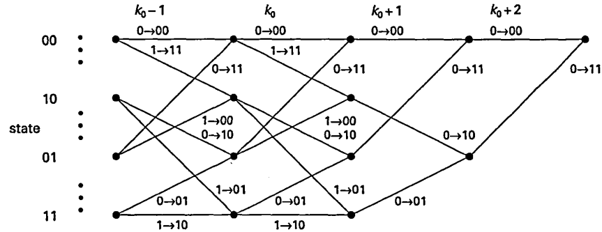
Figure 8.10. Trellis termination.
