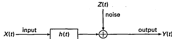
Figure 1.5. Linear Gaussian channel model.
