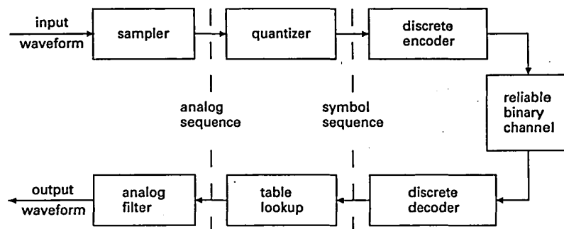
Figure 4.1. Encoding and decoding a waveform source.
