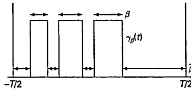
Figure 4.5. Let f(t) have the value 1 on a set B and the value 0 elsewhere in [-T/2, T/2] . Then \int f(t) dt = \mu(B) . The complement \overline{B} of B is also illustrated, and it is seen that 1 - f(t) is 1 on the set \overline{B} and 0 elsewhere. Thus \int [1 - f(t)] dt = \mu(\overline{B}) , which must equal T - \mu(B) for integration to correspond to the area under a curve.
