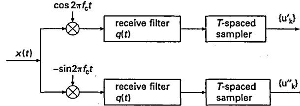
Figure 6.8. DSB-QC demodulation.
