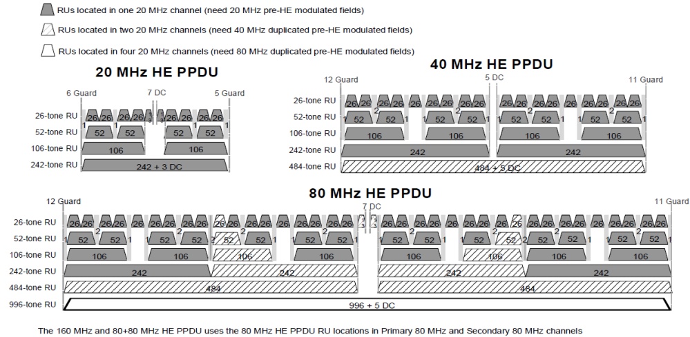
Figure 27-12—Number of 20 MHz channels occupied by the pre-HE modulated fields in an HE TB PDU
