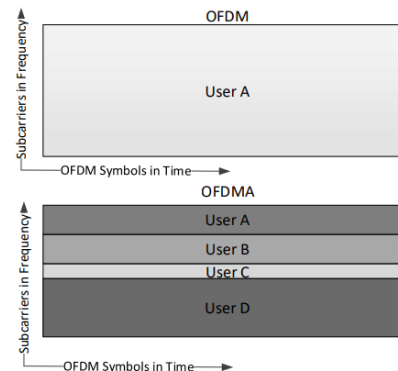
Figure 27-4—Illustration of OFDM and OFDMA concepts
