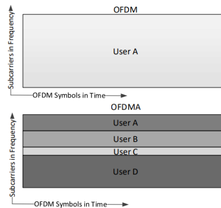
Figure 27-4—Illustration of OFDM and OFDMA concepts
