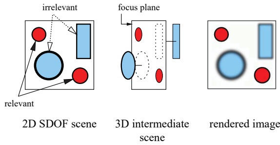
Figure 4. The photo-realistic camera and 2D SDOF.
