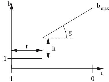
Figure 3. The Blur function.
