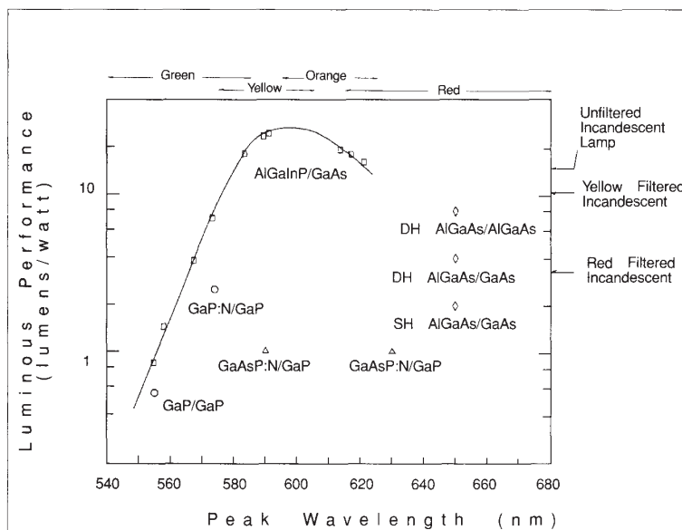
4. LED luminous performance versus wavelength for AlInGaP compared to other LED technologies. Luminous performance is the product of power efficiency (roughly equal to quantum efficiency), and the eye's response.
