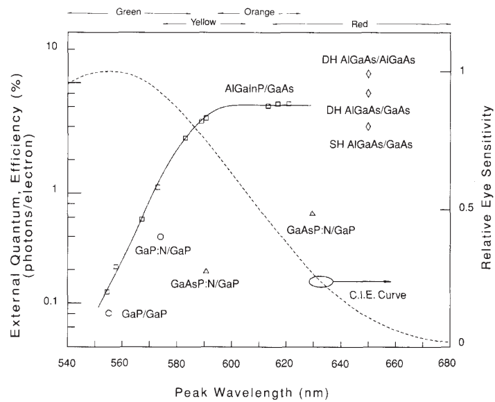
3. External quantum efficiency as a function of peak emission wavelength for AlInGaP devices. For red and yellow wavelengths beyond 590 nm, the devices have 5 percent efficiency. The efficiency drops at shorter wavelengths due to the approaching transition from a direct to an indirect semiconductor. The CIE eye-response curve is also shown.
