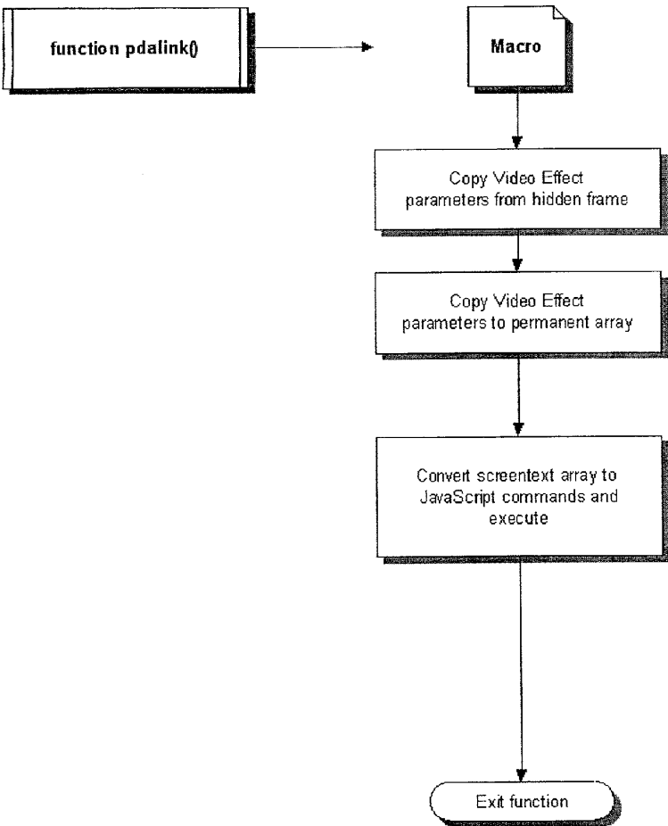
MatrixPlayer - Chart 5b: function pdalink(), datamode = "Macro"
