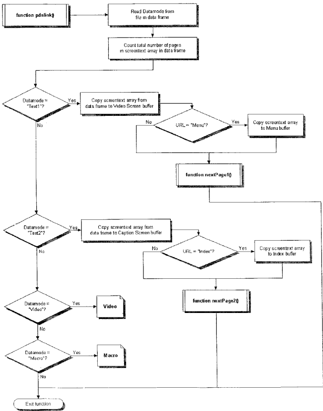
MatrixPlayer - Chart 5: function pdalink()
