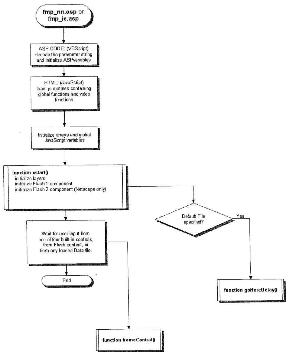
MatrixPlayer - Chart 2: Program Initialization and Overview
