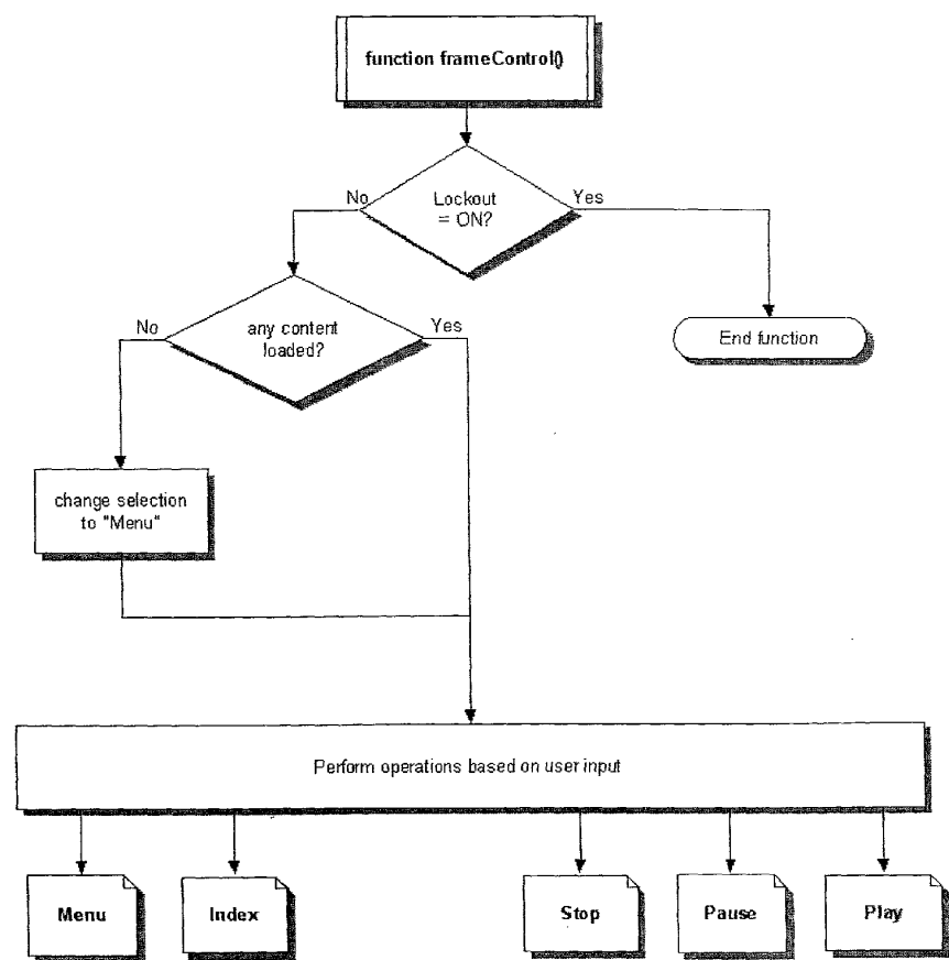
MatrixPlayer - Chart 3: function frameControl() overview
