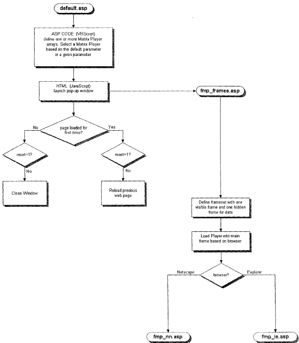
MatrixPlayer - Chart 1: Startup and File Structure
