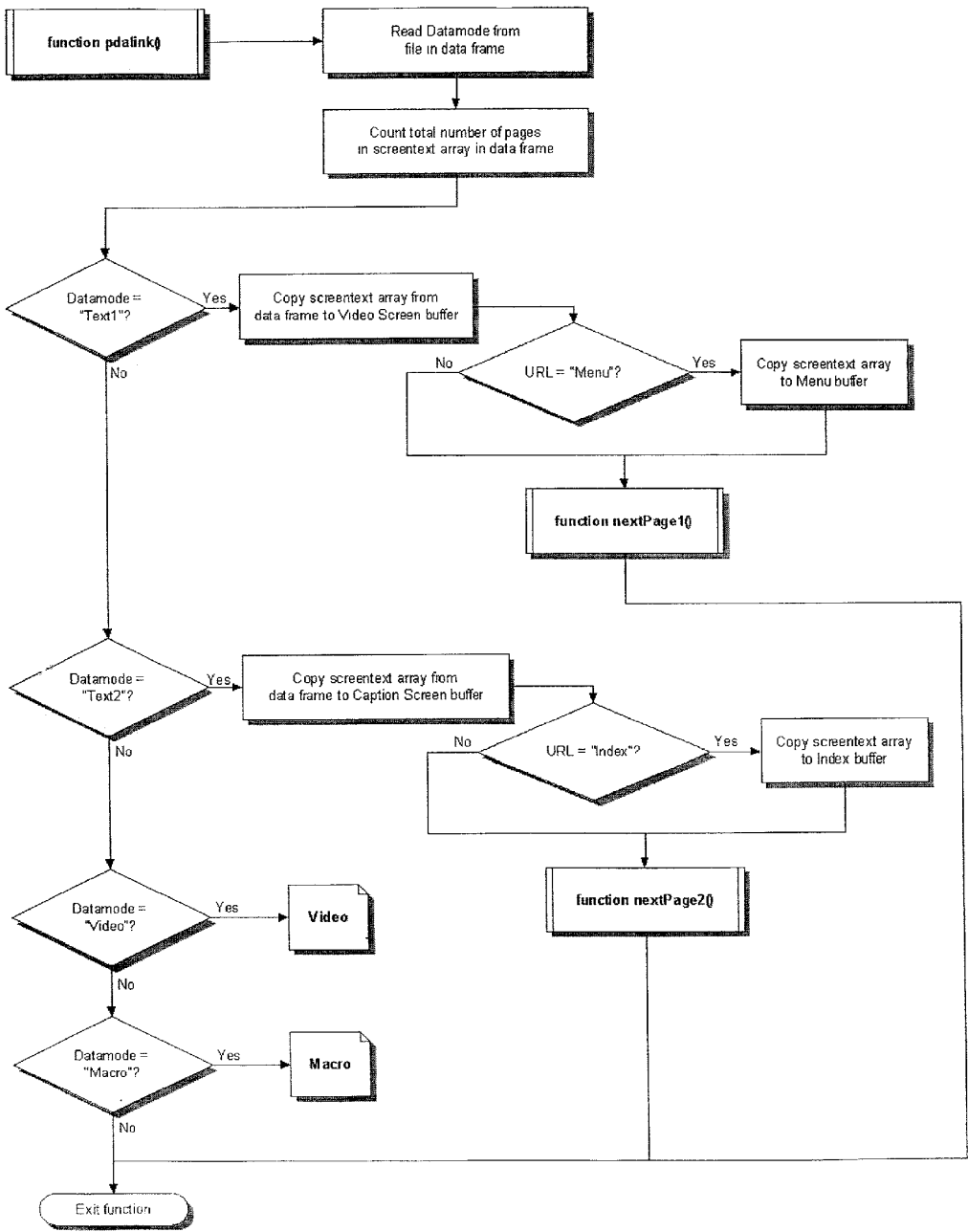
MatrixPlayer - Chart 5: function pdalink()
