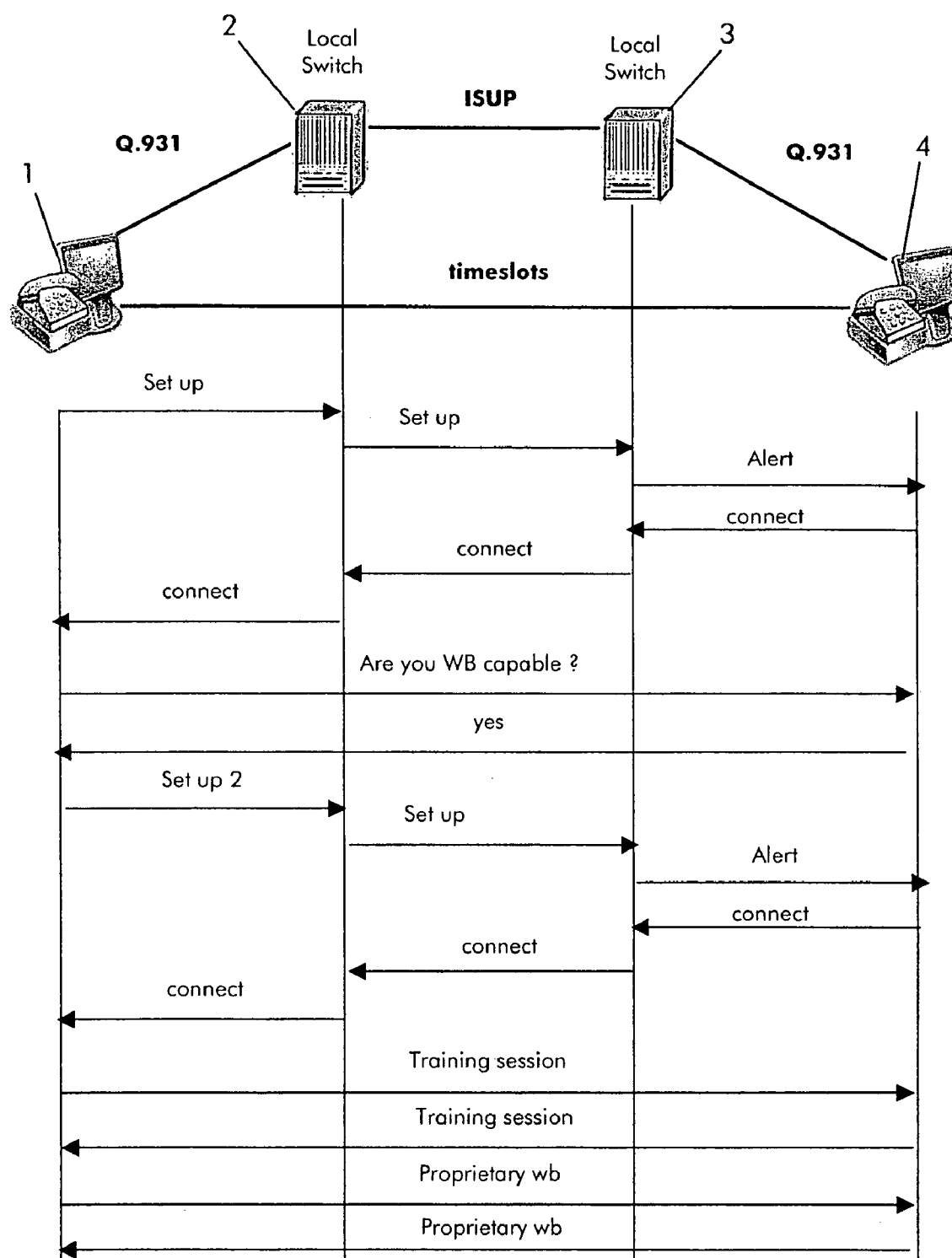
Fig. 1 (prior art)
