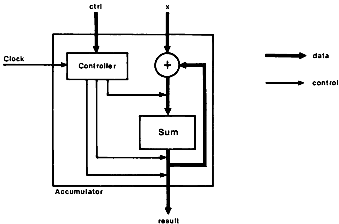
Figure 2-1: A hardware implementation of Accumulator
