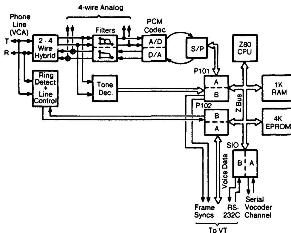
Figure 7-2: STN interface functional diagram
