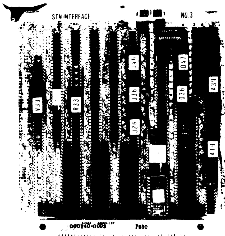
Figure 7-1: STN interface card
