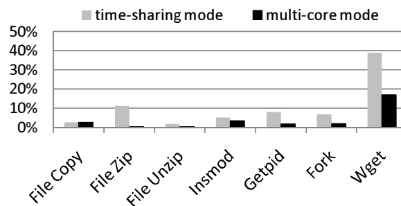
Figure 6: Performance overhead of an isolated VM compared with original Qemu/KVM
