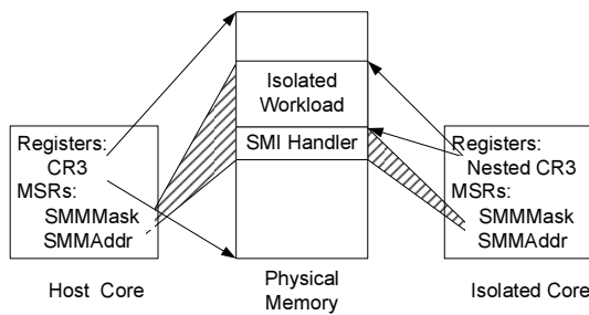
Figure 4: Double view of memory from different processor cores. From the host core's view, the isolated environment is part of the SMRAM. From the isolated workload's view, the SMI handler is protected by the SMRAM and the legacy host is protected by the security manager via hardware assisted paging.
