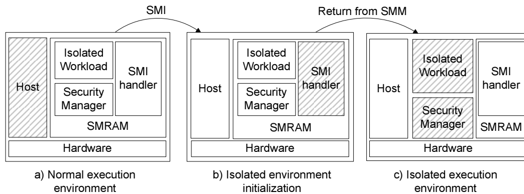
Figure 2: Entering SICE from the legacy host (actively running components are shaded): a) An SMI triggers SICE operations. b) The SMI handler prepares the isolated environment and the new SMRAM layout. c) After entering the isolated environment, the security manager prevents the isolated workload from accessing the legacy host memory.
