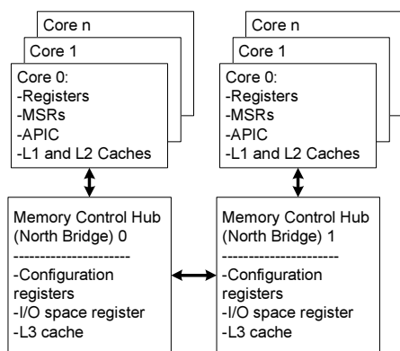
Figure 3: General multi-core processors architecture
