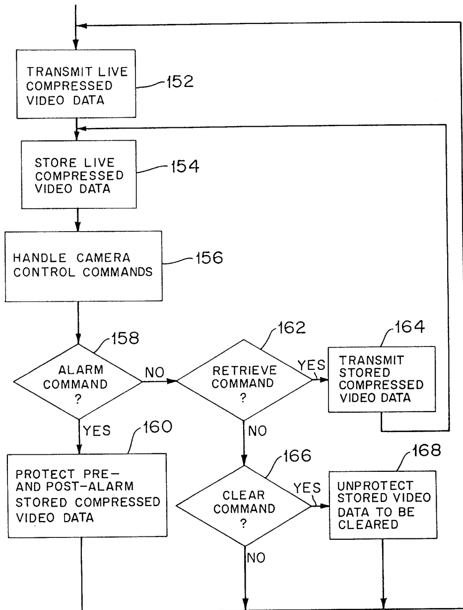
FIG. 4 CAMERA UNIT OPERATION
